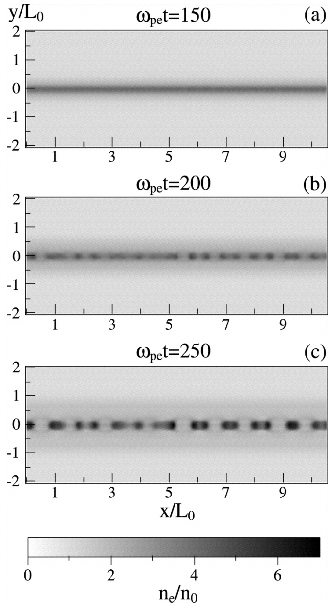
Fig. 5. from A Trigger Mechanism of Magnetic Reconnection and Particle Acceleration during Thinning of the Current Sheet Saito & Sakai 2006 ApJ 652 793 doi:10.1086/508333 https://dx.doi.org/10.1086/508333
