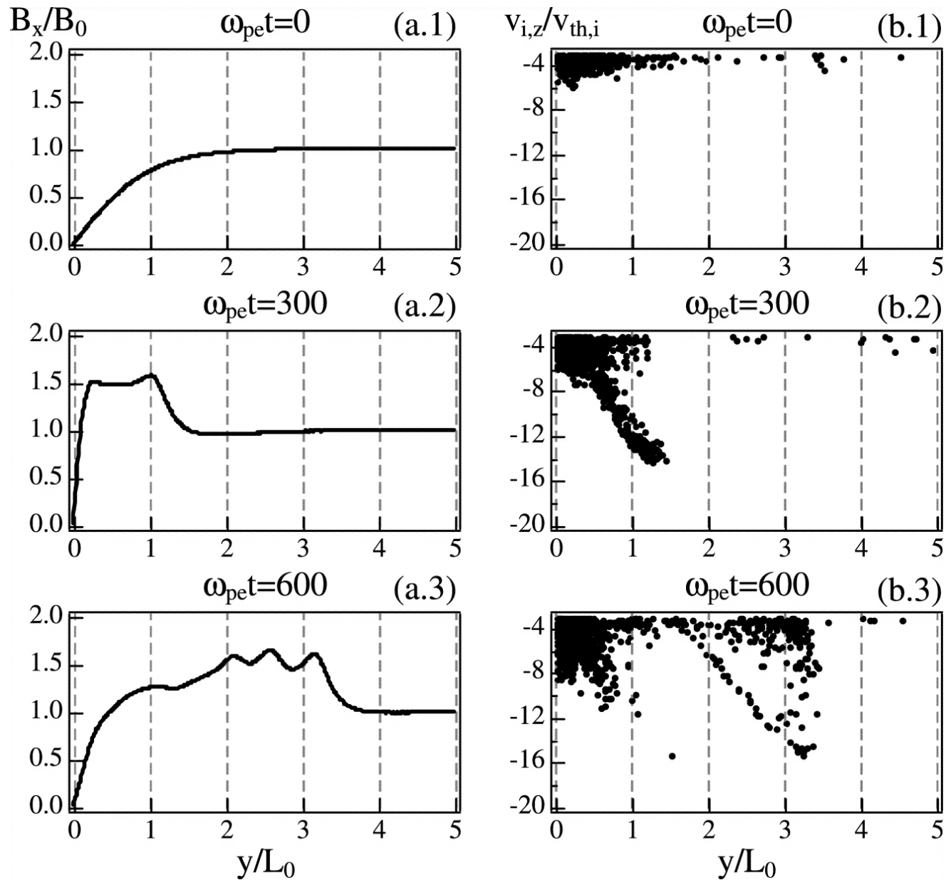
Fig. 4. from A Trigger Mechanism of Magnetic Reconnection and Particle Acceleration during Thinning of the Current Sheet Saito & Sakai 2006 ApJ 652 793 doi:10.1086/508333 https://dx.doi.org/10.1086/508333
