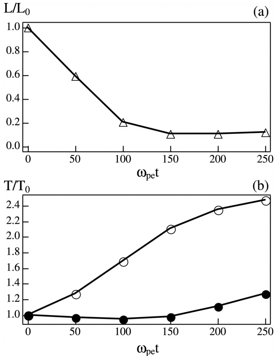
Fig. 3. from A Trigger Mechanism of Magnetic Reconnection and Particle Acceleration during Thinning of the Current Sheet Saito & Sakai 2006 ApJ 652 793 doi:10.1086/508333 https://dx.doi.org/10.1086/508333
