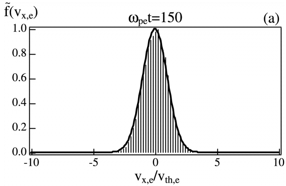
Fig. 2. from A Trigger Mechanism of Magnetic Reconnection and Particle Acceleration during Thinning of the Current Sheet Saito & Sakai 2006 ApJ 652 793 doi:10.1086/508333 https://dx.doi.org/10.1086/508333
