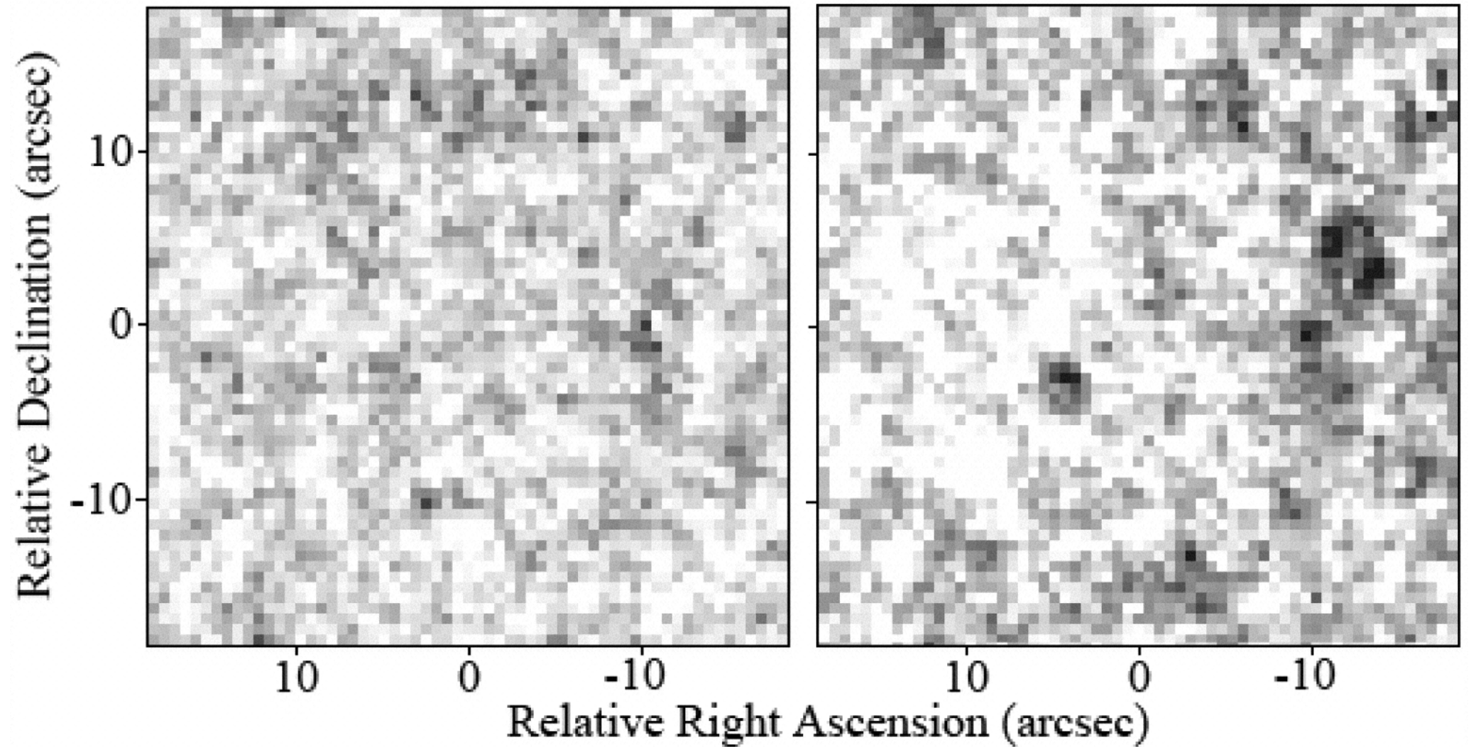
Fig. 8. from Deep ATLAS Radio Observations of the Chandra Deep Field–South/Spitzer WideArea Infrared Extragalactic Field Norris et al. 2006 AJ 132 2409 doi:10.1086/508275 https://dx.doi.org/10.1086/508275 © 2006. The American Astronomical Society. All rights reserved. Printed in U.S.A.
