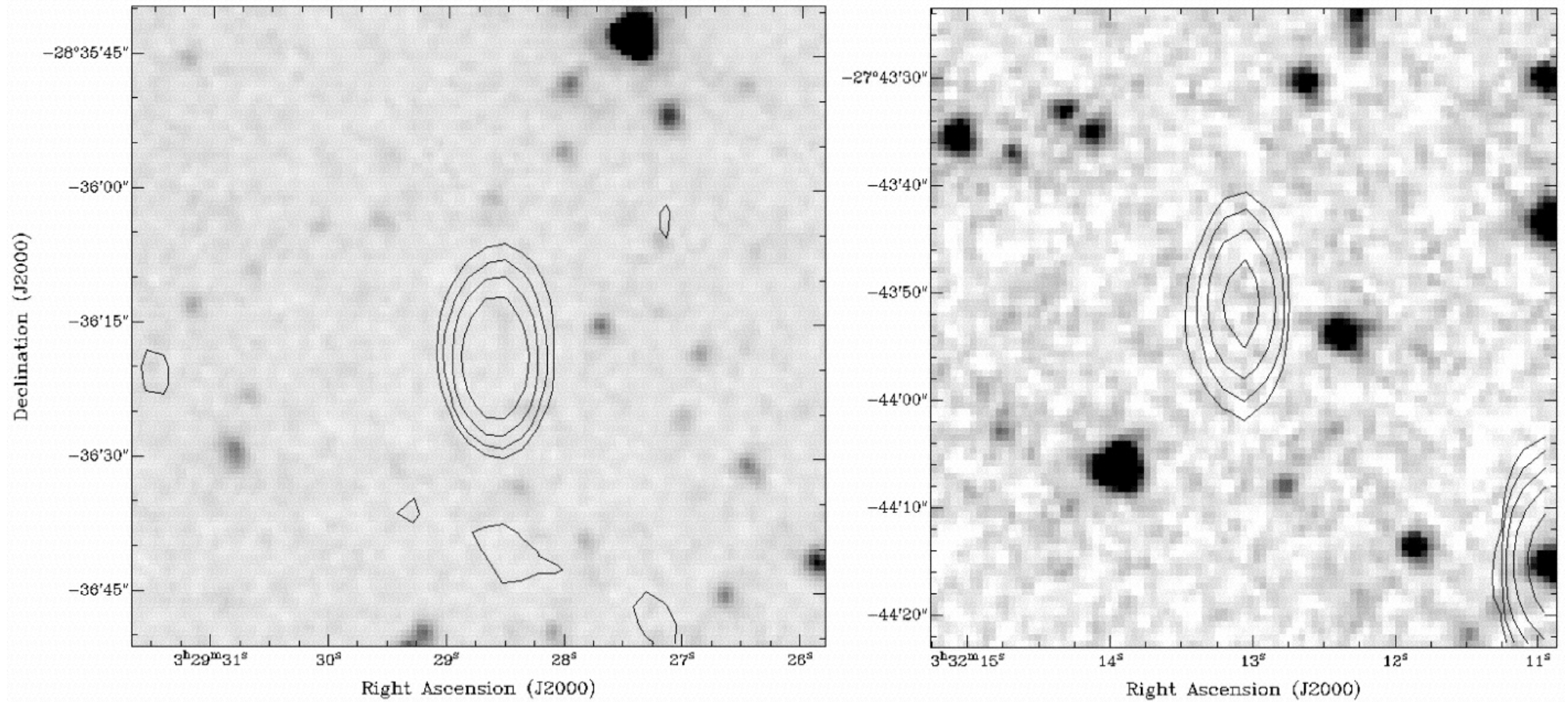
Fig. 7. from Deep ATLAS Radio Observations of the Chandra Deep Field–South/Spitzer WideArea Infrared Extragalactic Field Norris et al. 2006 AJ 132 2409 doi:10.1086/508275 https://dx.doi.org/10.1086/508275 © 2006. The American Astronomical Society. All rights reserved. Printed in U.S.A.
