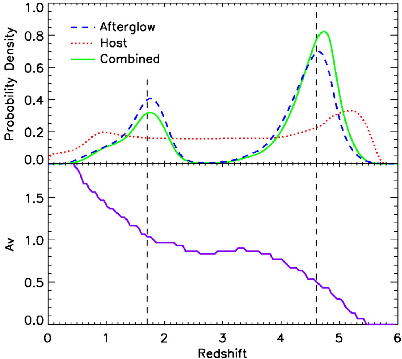
Fig. 4. from GRB 060121: Implications of a Short/IntermediateDuration Ray Burst at High Redshift de Ugarte Postigo et al. 2006 ApJL 648 L83 doi:10.1086/507868 https://dx.doi.org/10.1086/507868
