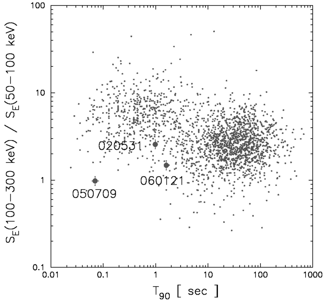
Fig. 3. from GRB 060121: Implications of a Short/IntermediateDuration Ray Burst at High Redshift de Ugarte Postigo et al. 2006 ApJL 648 L83 doi:10.1086/507868 https://dx.doi.org/10.1086/507868
