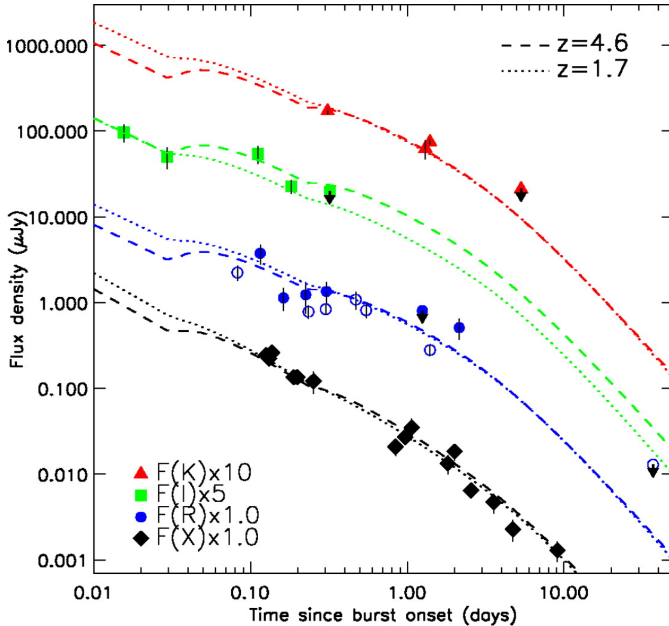
Fig. 2. from GRB 060121: Implications of a Short/IntermediateDuration Ray Burst at High Redshift de Ugarte Postigo et al. 2006 ApJL 648 L83 doi:10.1086/507868 https://dx.doi.org/10.1086/507868 © 2006. The American Astronomical Society. All rights reserved. Printed in U.S.A.
