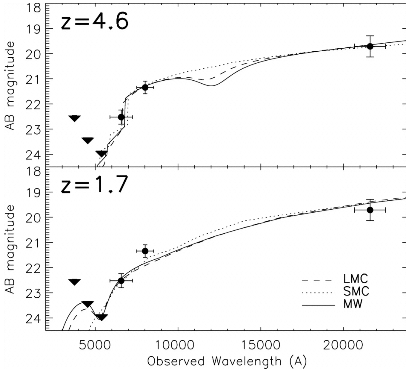
Fig. 1. from GRB 060121: Implications of a Short/IntermediateDuration Ray Burst at High Redshift de Ugarte Postigo et al. 2006 ApJL 648 L83 doi:10.1086/507868 https://dx.doi.org/10.1086/507868
