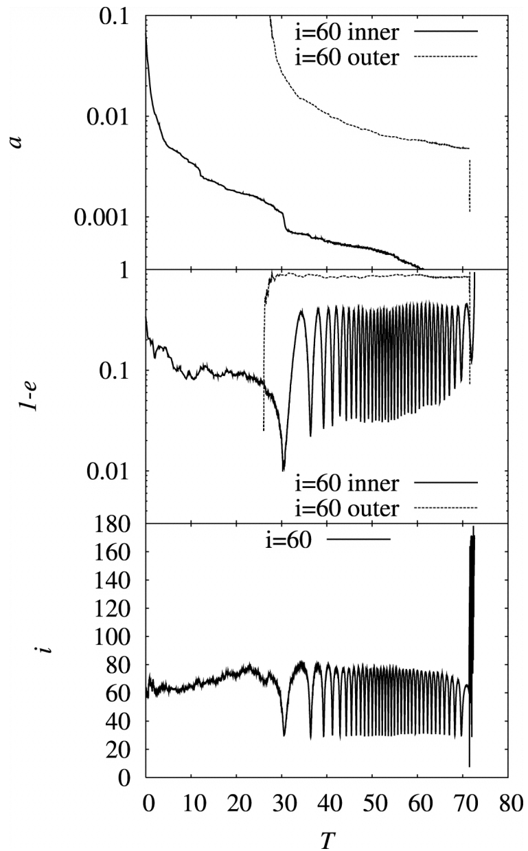
Fig. 8. from Evolution of Massive Black Hole Triples. I. EqualMass BinarySingle Systems Iwasawa, Funato, & Makino 2006 ApJ 651 1059 doi:10.1086/507473 https://dx.doi.org/10.1086/507473
