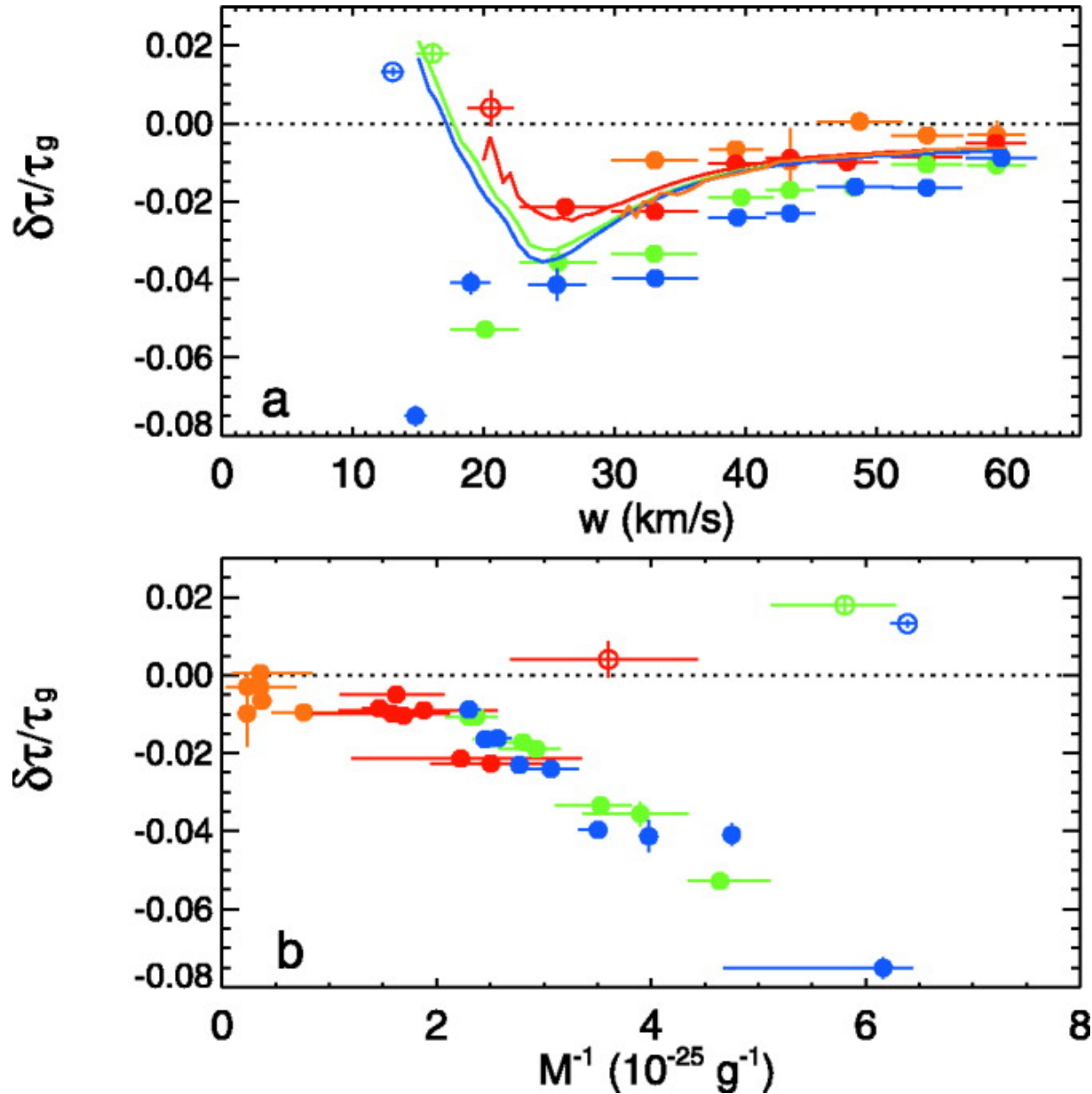
Fig. 3. from Observed Frequency Variations of Solar pMode Travel Times as Evidence for Surface Effects in Sunspot Seismology Braun & Birch 2006 ApJL 647 L187 doi:10.1086/507450 https://dx.doi.org/10.1086/507450 © 2006. The American Astronomical Society. All rights reserved. Printed in U.S.A.
