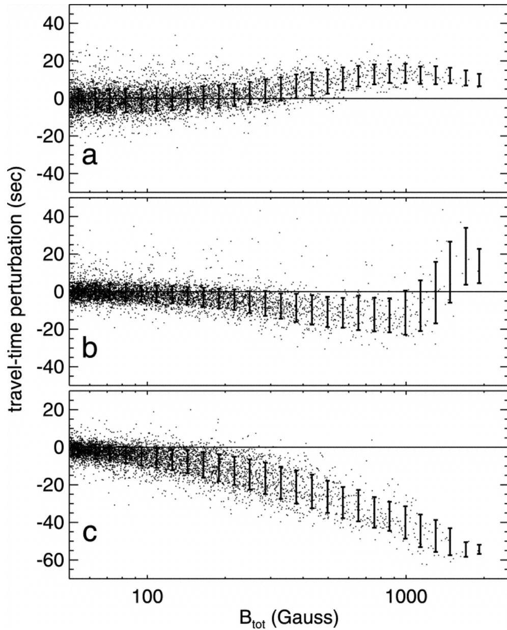
Fig. 2. from Observed Frequency Variations of Solar pMode Travel Times as Evidence for Surface Effects in Sunspot Seismology Braun & Birch 2006 ApJL 647 L187 doi:10.1086/507450 https://dx.doi.org/10.1086/507450
