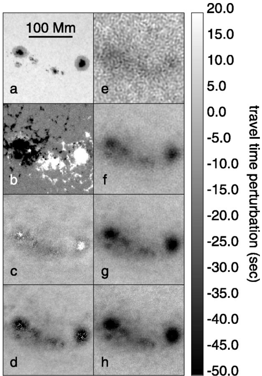
Fig. 1. from Observed Frequency Variations of Solar pMode Travel Times as Evidence for Surface Effects in Sunspot Seismology Braun & Birch 2006 ApJL 647 L187 doi:10.1086/507450 https://dx.doi.org/10.1086/507450
