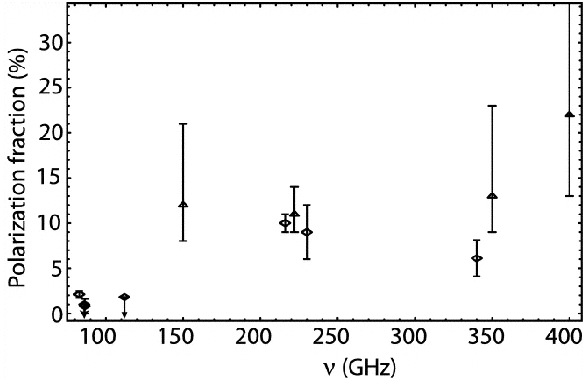
Fig. 3. from The Rotation Measure and 3.5 Millimeter Polarization of Sagittarius A* Macquart et al. 2006 ApJL 646 L111 doi:10.1086/506932 https://dx.doi.org/10.1086/506932 © 2006. The American Astronomical Society. All rights reserved. Printed in U.S.A.
