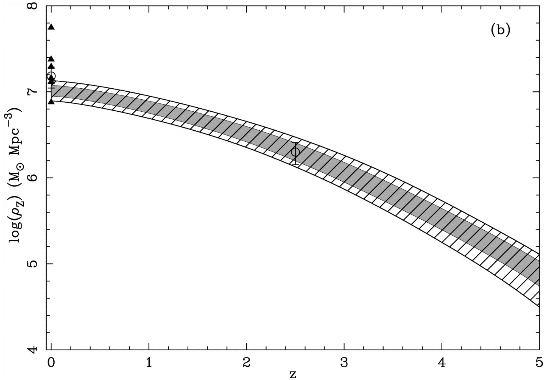
Fig. 6. from On the Normalization of the Cosmic Star Formation History Hopkins & Beacom 2006 ApJ 651 142 doi:10.1086/506610 https://dx.doi.org/10.1086/506610 © 2006. The American Astronomical Society. All rights reserved. Printed in U.S.A.
