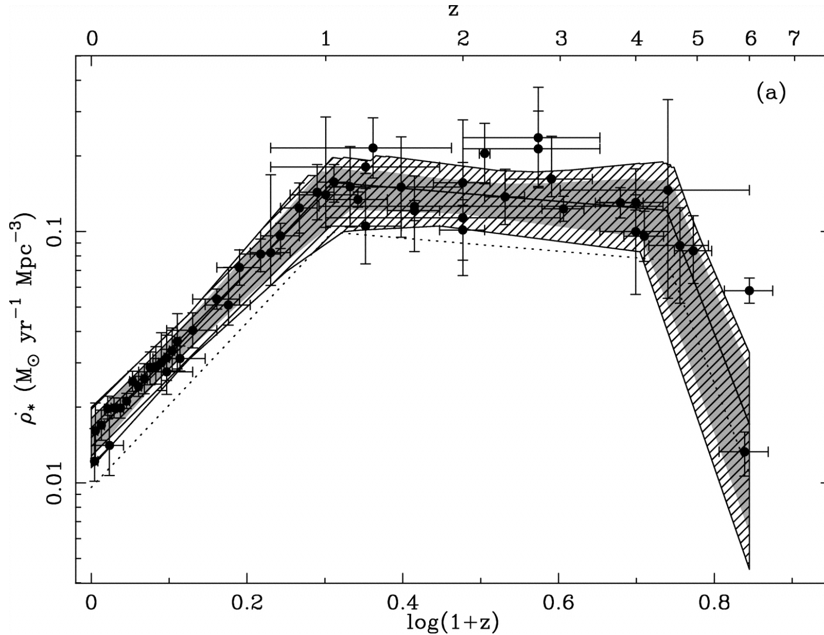
Fig. 4. from On the Normalization of the Cosmic Star Formation History Hopkins & Beacom 2006 ApJ 651 142 doi:10.1086/506610 https://dx.doi.org/10.1086/506610 © 2006. The American Astronomical Society. All rights reserved. Printed in U.S.A.
