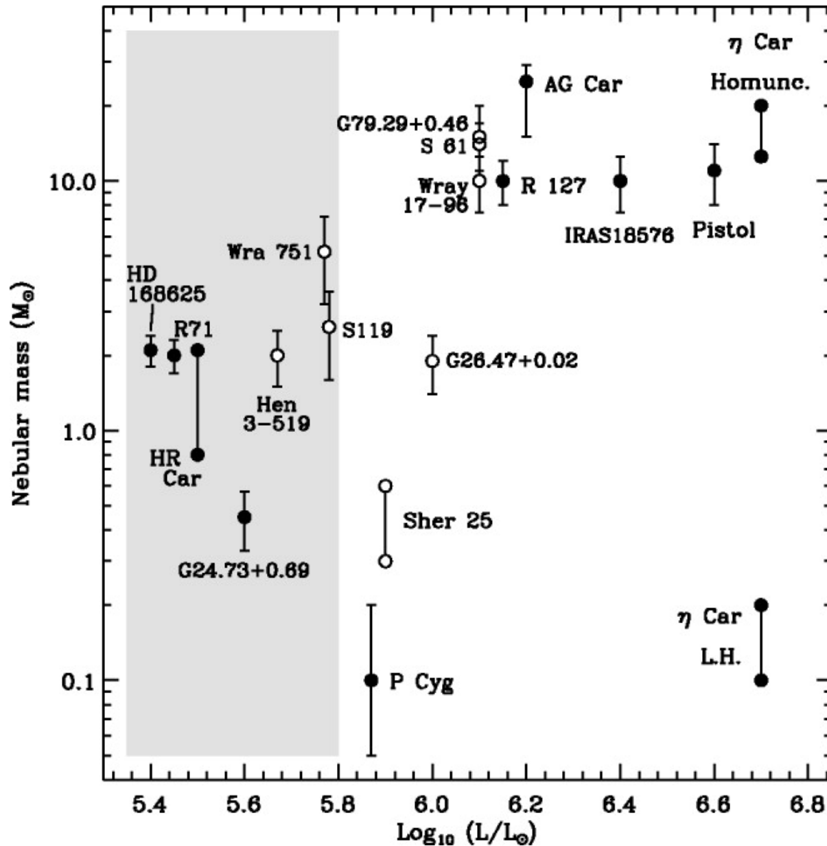
Fig. 1. from On the Role of Continuumdriven Eruptions in the Evolution of Very Massive Stars and Population III Stars Smith & Owocki 2006 ApJL 645 L45 doi:10.1086/506523 https://dx.doi.org/10.1086/506523 © 2006. The American Astronomical Society. All rights reserved. Printed in U.S.A.
