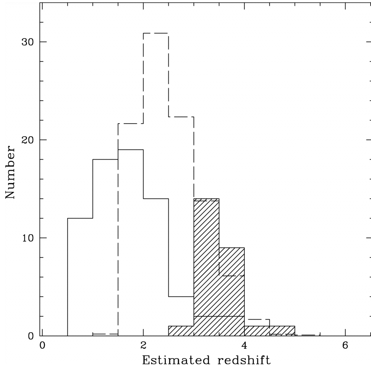
Fig. 8. from The DRaGONS Survey: A Search for HighRedshift Radio Galaxies and Heavily Obscured Active Galactic Nuclei Schmidt, Connolly, & Hopkins 2006 ApJ 649 63 doi:10.1086/506444 https://dx.doi.org/10.1086/506444 © 2006. The American Astronomical Society. All rights reserved. Printed in U.S.A.
