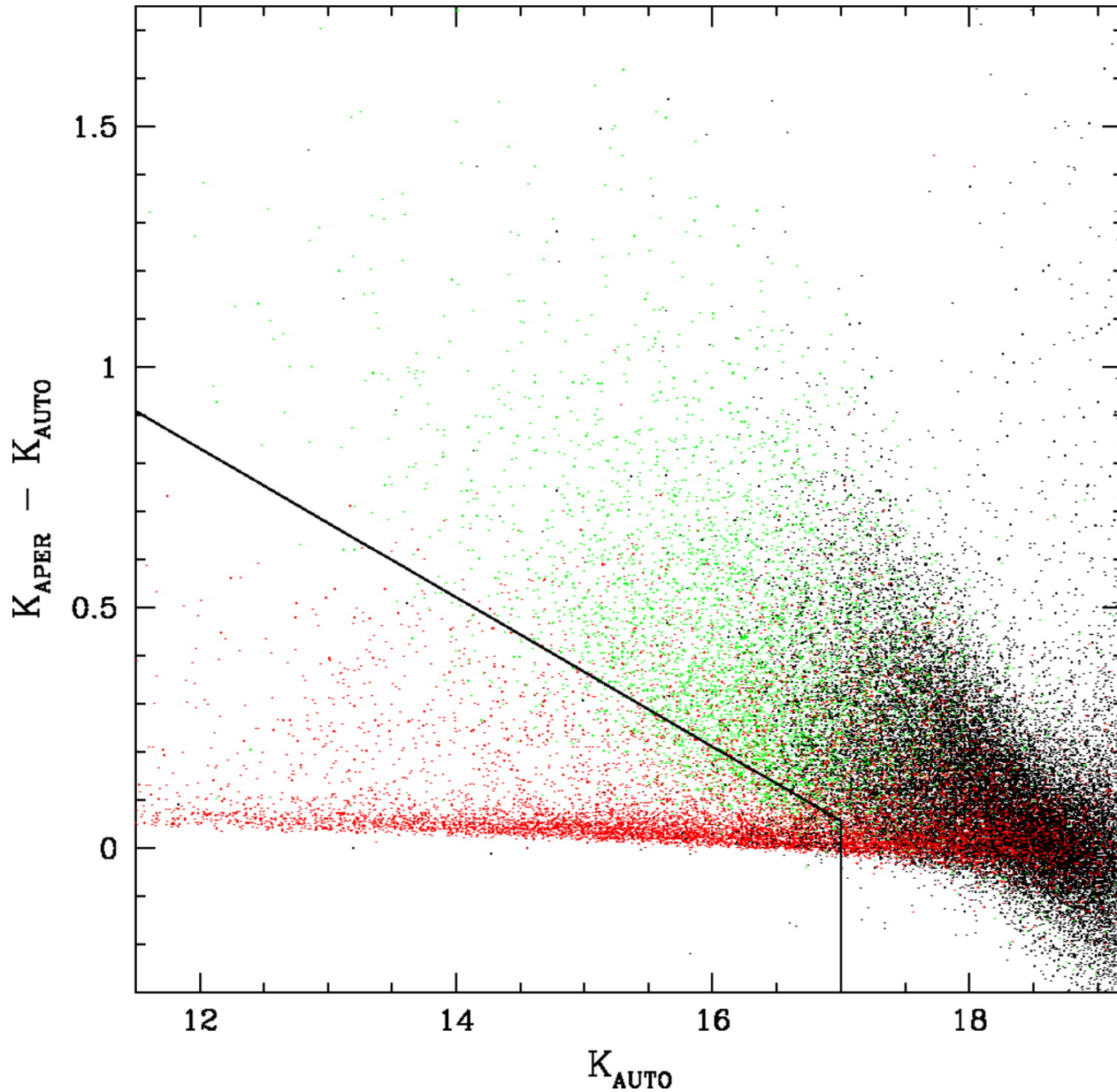
Fig. 5. from The DRaGONS Survey: A Search for HighRedshift Radio Galaxies and Heavily Obscured Active Galactic Nuclei Schmidt, Connolly, & Hopkins 2006 ApJ 649 63 doi:10.1086/506444 https://dx.doi.org/10.1086/506444
