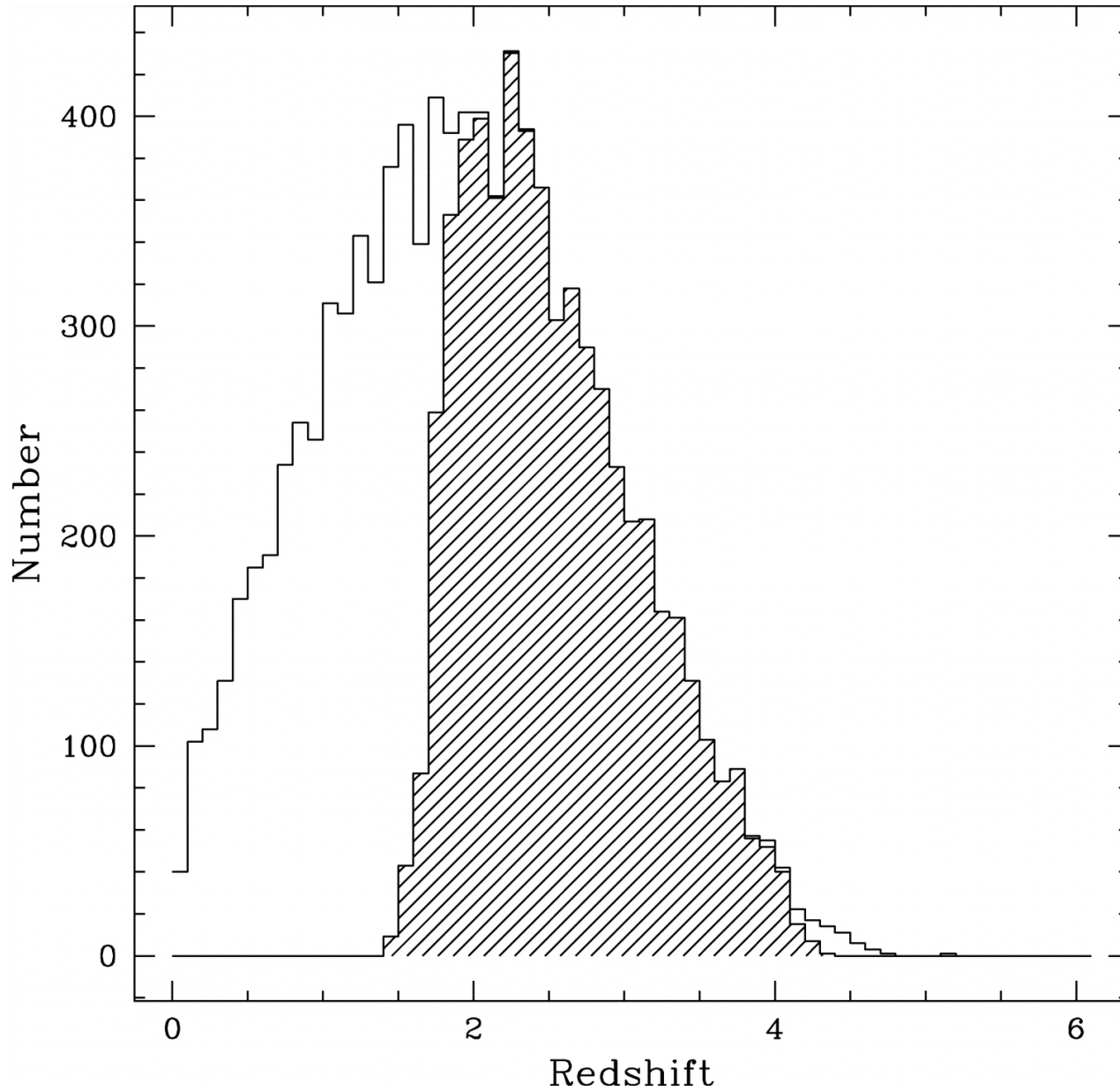
Fig. 3. from The DRaGONS Survey: A Search for HighRedshift Radio Galaxies and Heavily Obscured Active Galactic Nuclei Schmidt, Connolly, & Hopkins 2006 ApJ 649 63 doi:10.1086/506444 https://dx.doi.org/10.1086/506444
