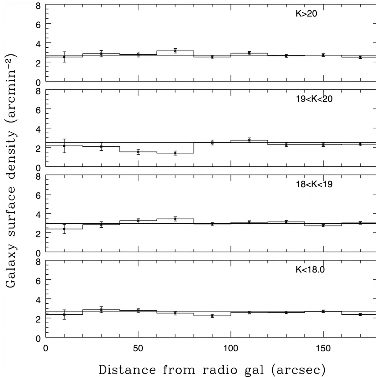
Fig. 16. from The DRaGONS Survey: A Search for HighRedshift Radio Galaxies and Heavily Obscured Active Galactic Nuclei Schmidt, Connolly, & Hopkins 2006 ApJ 649 63 doi:10.1086/506444 https://dx.doi.org/10.1086/506444
