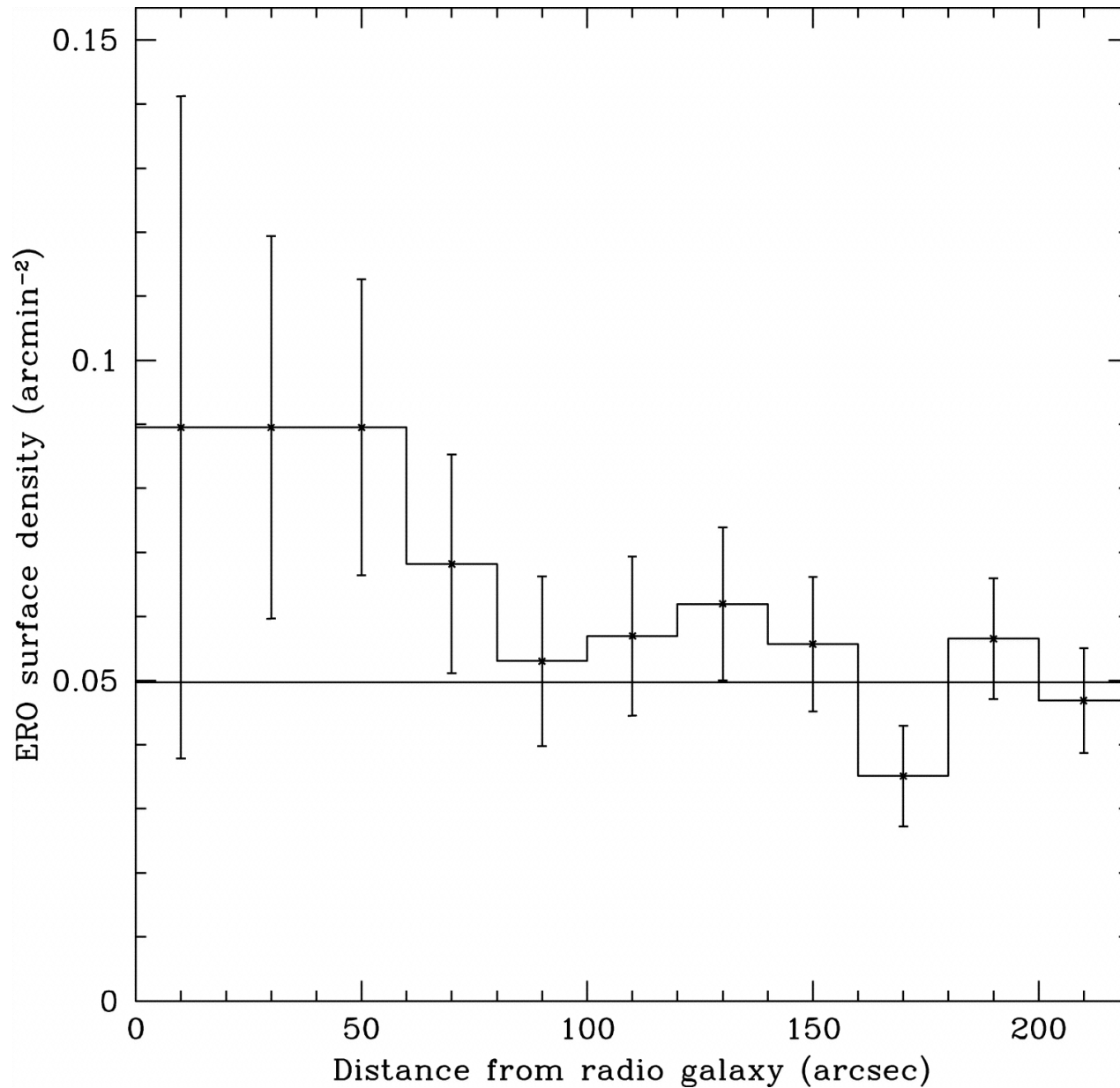
Fig. 15. from The DRaGONS Survey: A Search for HighRedshift Radio Galaxies and Heavily Obscured Active Galactic Nuclei Schmidt, Connolly, & Hopkins 2006 ApJ 649 63 doi:10.1086/506444 https://dx.doi.org/10.1086/506444
