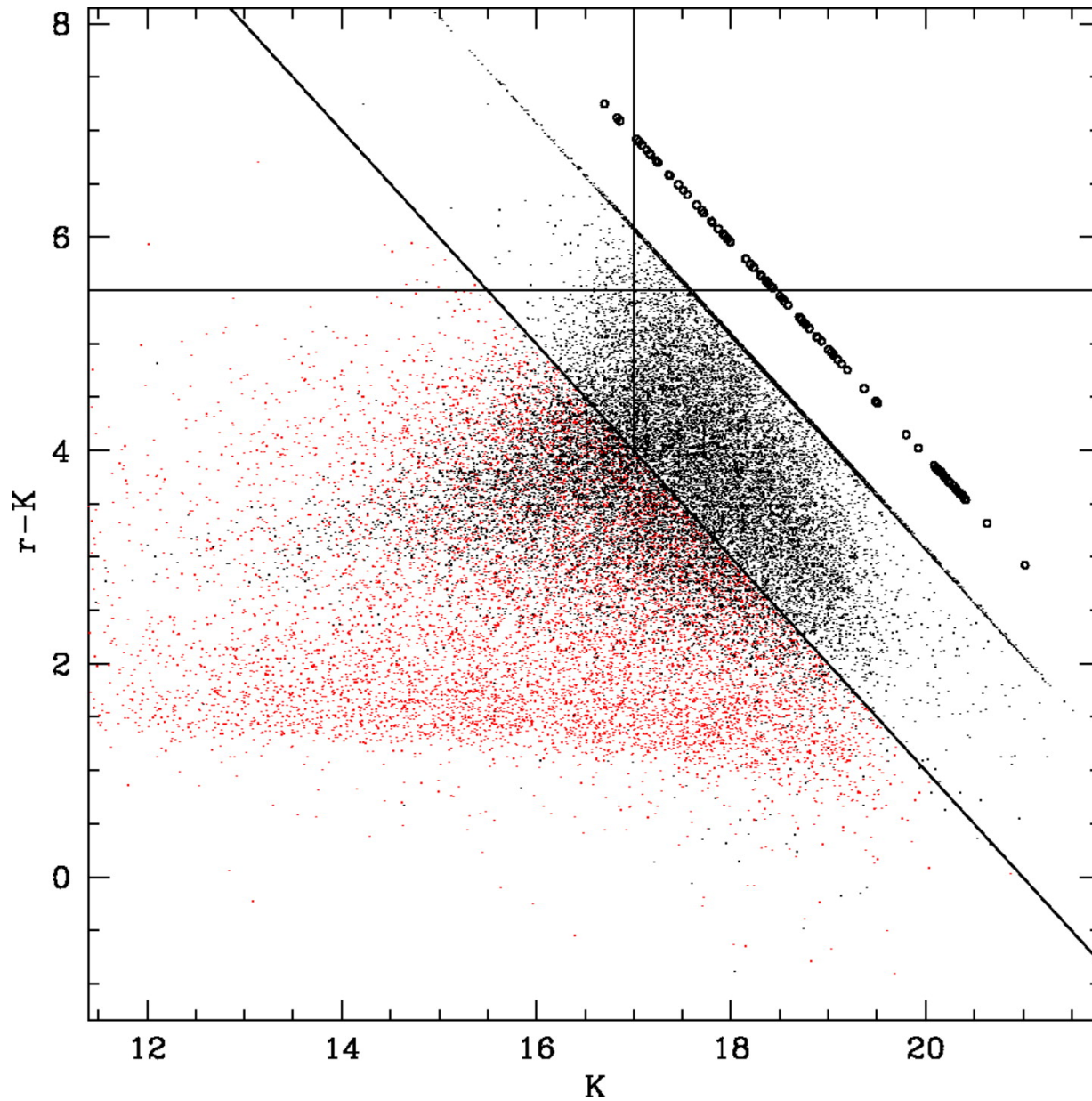
Fig. 13. from The DRaGONS Survey: A Search for HighRedshift Radio Galaxies and Heavily Obscured Active Galactic Nuclei Schmidt, Connolly, & Hopkins 2006 ApJ 649 63 doi:10.1086/506444 https://dx.doi.org/10.1086/506444
