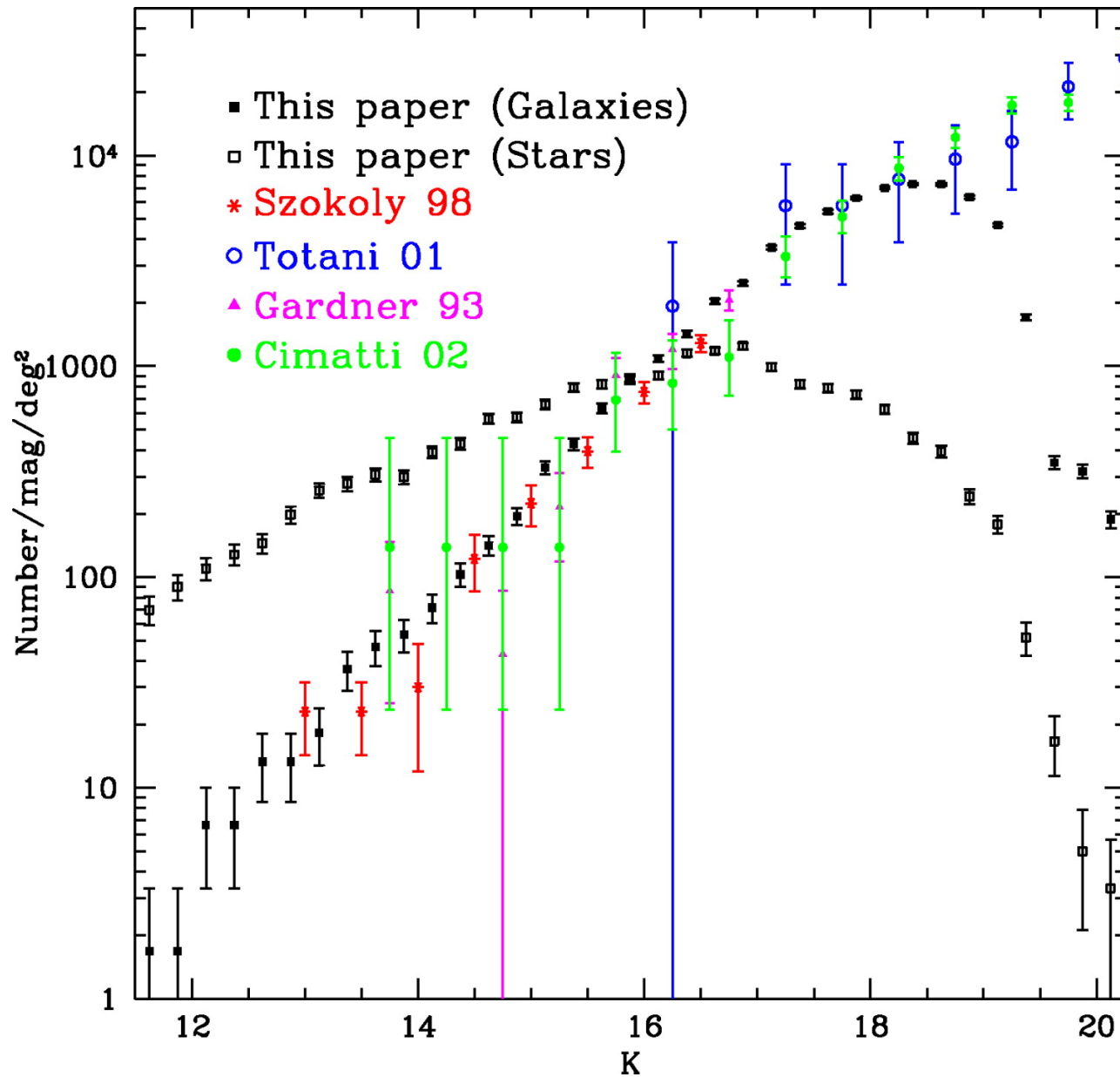
Fig. 12. from The DRaGONS Survey: A Search for HighRedshift Radio Galaxies and Heavily Obscured Active Galactic Nuclei Schmidt, Connolly, & Hopkins 2006 ApJ 649 63 doi:10.1086/506444 https://dx.doi.org/10.1086/506444 © 2006. The American Astronomical Society. All rights reserved. Printed in U.S.A.
