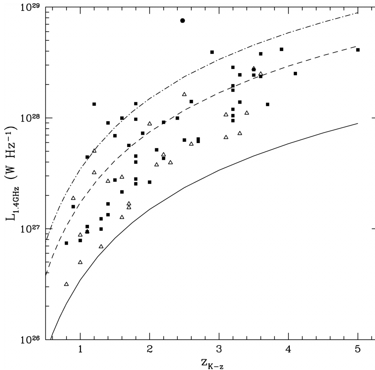
Fig. 11. from The DRaGONS Survey: A Search for HighRedshift Radio Galaxies and Heavily Obscured Active Galactic Nuclei Schmidt, Connolly, & Hopkins 2006 ApJ 649 63 doi:10.1086/506444 https://dx.doi.org/10.1086/506444
