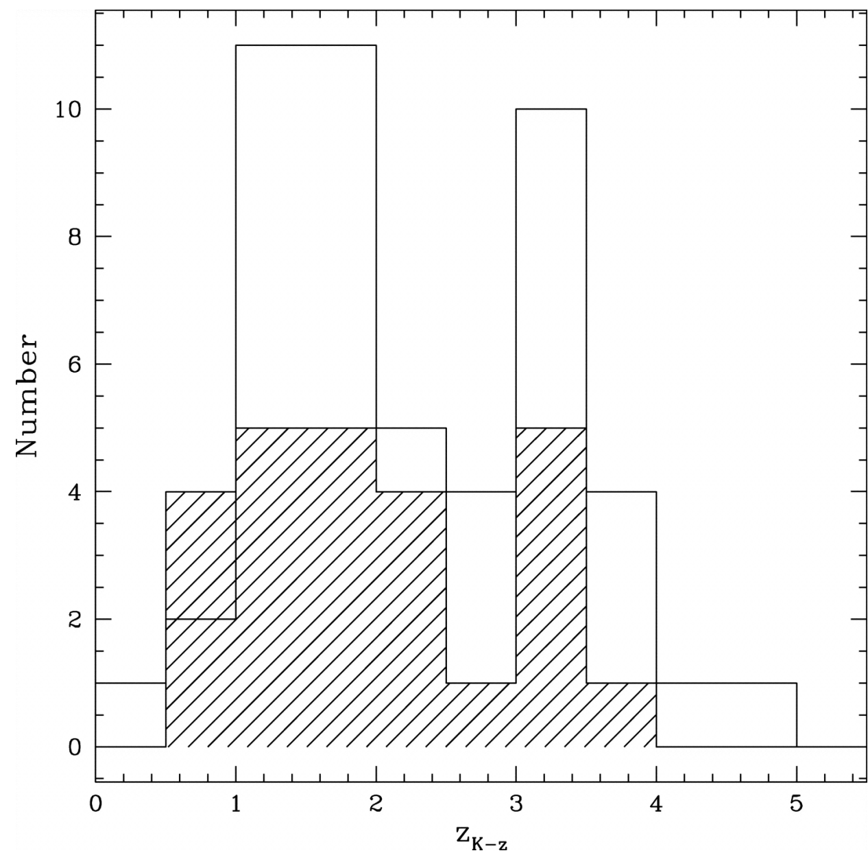
Fig. 10. from The DRaGONS Survey: A Search for HighRedshift Radio Galaxies and Heavily Obscured Active Galactic Nuclei Schmidt, Connolly, & Hopkins 2006 ApJ 649 63 doi:10.1086/506444 https://dx.doi.org/10.1086/506444 © 2006. The American Astronomical Society. All rights reserved. Printed in U.S.A.
