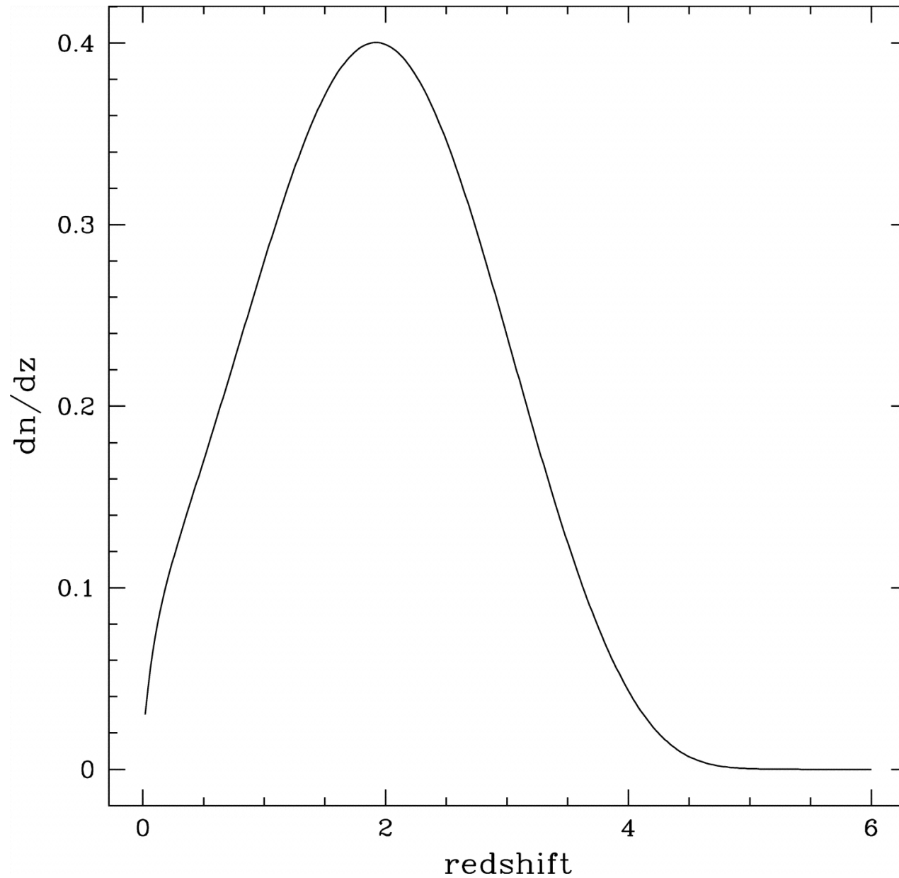
Fig. 1. from The DRaGONS Survey: A Search for HighRedshift Radio Galaxies and Heavily Obscured Active Galactic Nuclei Schmidt, Connolly, & Hopkins 2006 ApJ 649 63 doi:10.1086/506444 https://dx.doi.org/10.1086/506444
