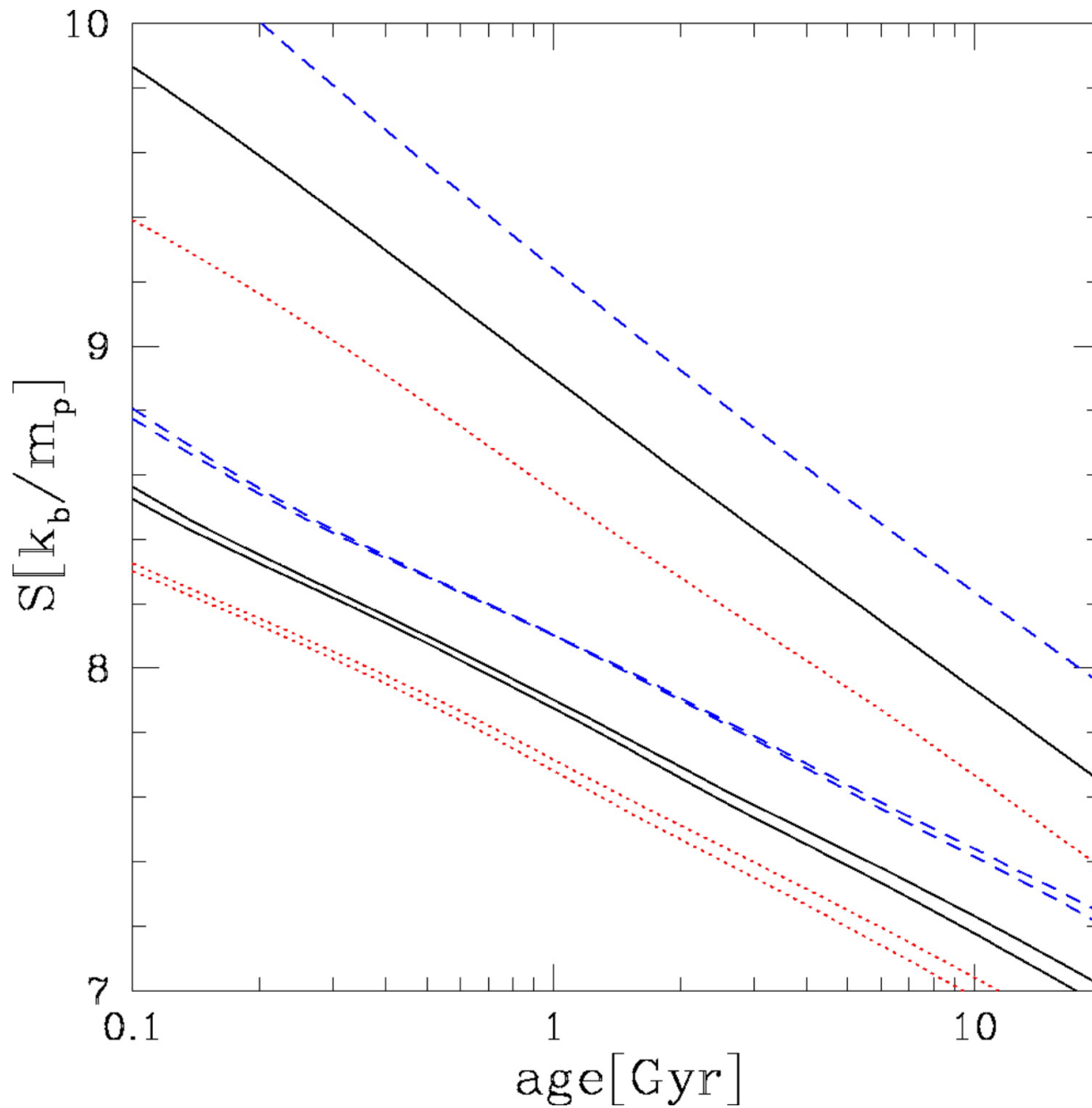
Fig. 9. from Thermal Structure and Radius Evolution of Irradiated Gas Giant Planets Arras & Bildsten 2006 ApJ 650 394 doi:10.1086/506011 https://dx.doi.org/10.1086/506011
