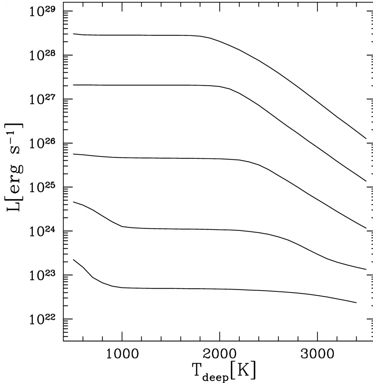
Fig. 4. from Thermal Structure and Radius Evolution of Irradiated Gas Giant Planets Arras & Bildsten 2006 ApJ 650 394 doi:10.1086/506011 https://dx.doi.org/10.1086/506011 © 2006. The American Astronomical Society. All rights reserved. Printed in U.S.A.
