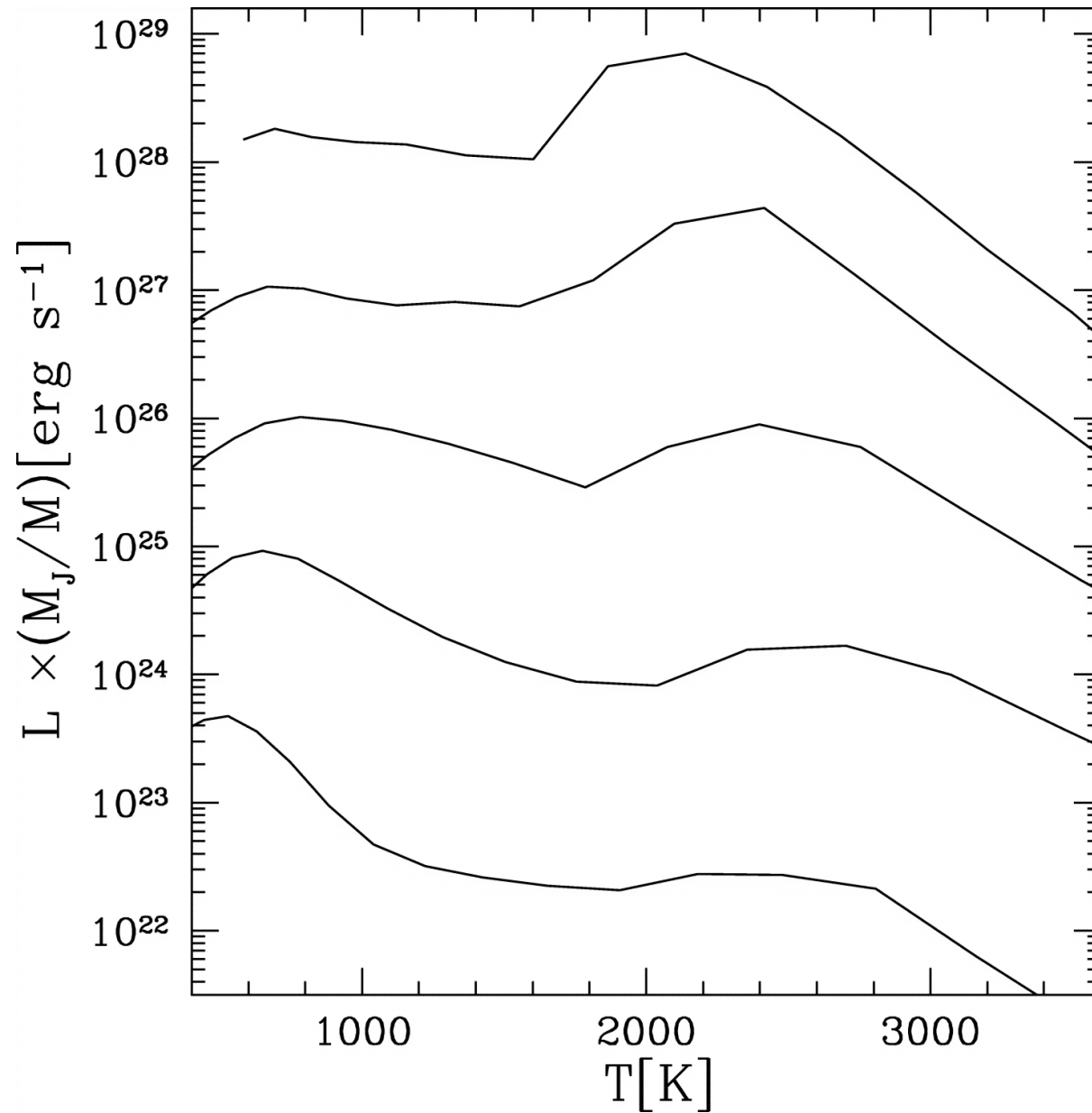
Fig. 3. from Thermal Structure and Radius Evolution of Irradiated Gas Giant Planets Arras & Bildsten 2006 ApJ 650 394 doi:10.1086/506011 https://dx.doi.org/10.1086/506011 © 2006. The American Astronomical Society. All rights reserved. Printed in U.S.A.
