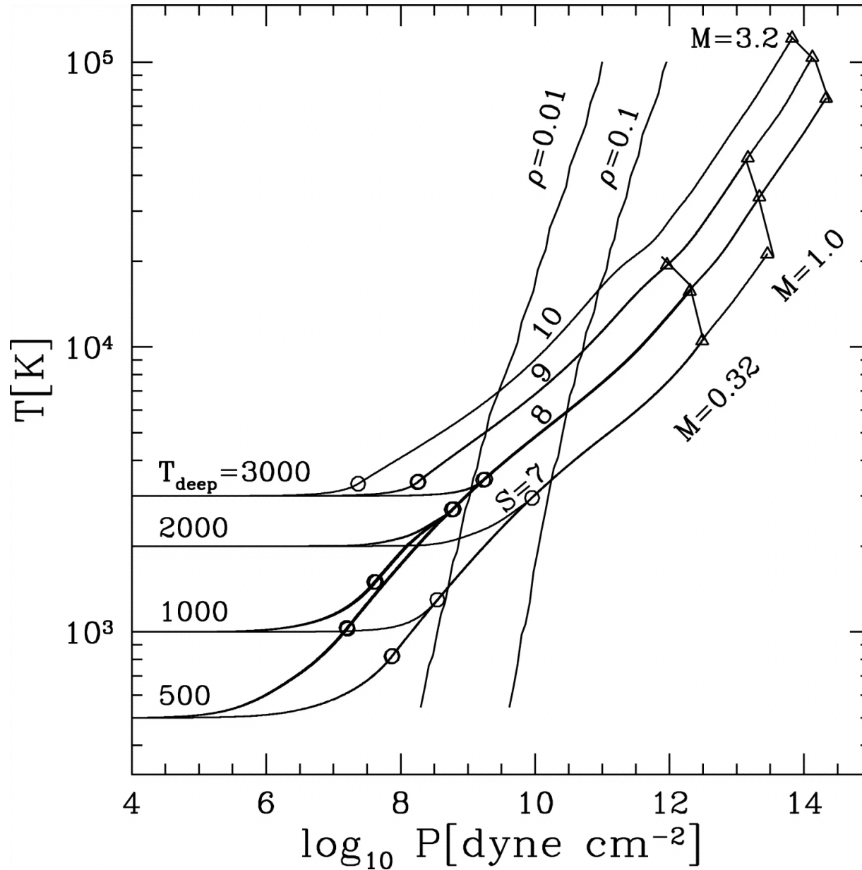
Fig. 2. from Thermal Structure and Radius Evolution of Irradiated Gas Giant Planets Arras & Bildsten 2006 ApJ 650 394 doi:10.1086/506011 https://dx.doi.org/10.1086/506011 © 2006. The American Astronomical Society. All rights reserved. Printed in U.S.A.
