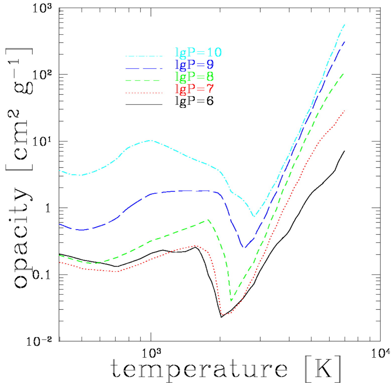
Fig. 1. from Thermal Structure and Radius Evolution of Irradiated Gas Giant Planets Arras & Bildsten 2006 ApJ 650 394 doi:10.1086/506011 https://dx.doi.org/10.1086/506011 © 2006. The American Astronomical Society. All rights reserved. Printed in U.S.A.
