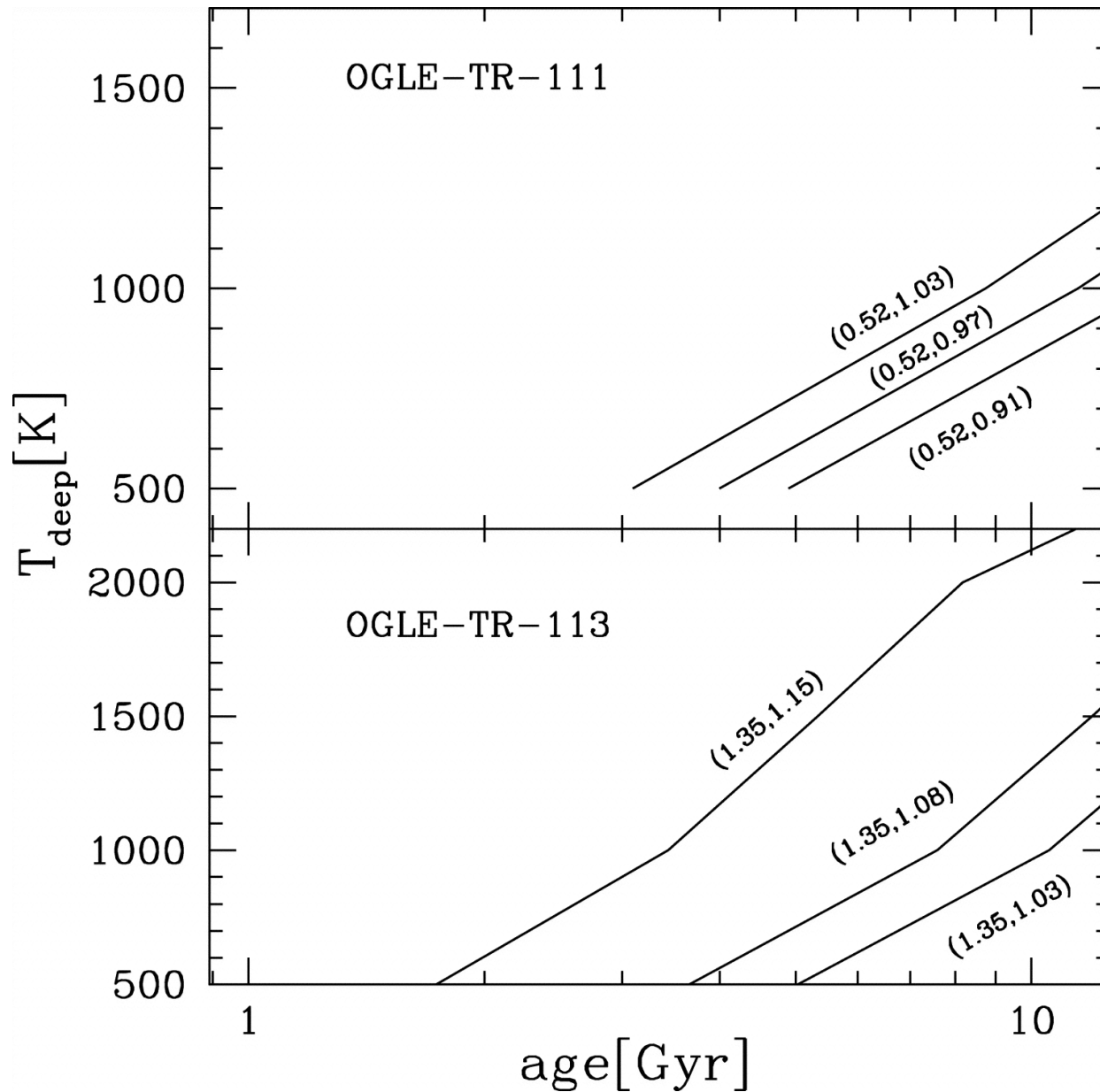
Fig. 19. from Thermal Structure and Radius Evolution of Irradiated Gas Giant Planets Arras & Bildsten 2006 ApJ 650 394 doi:10.1086/506011 https://dx.doi.org/10.1086/506011 © 2006. The American Astronomical Society. All rights reserved. Printed in U.S.A.
