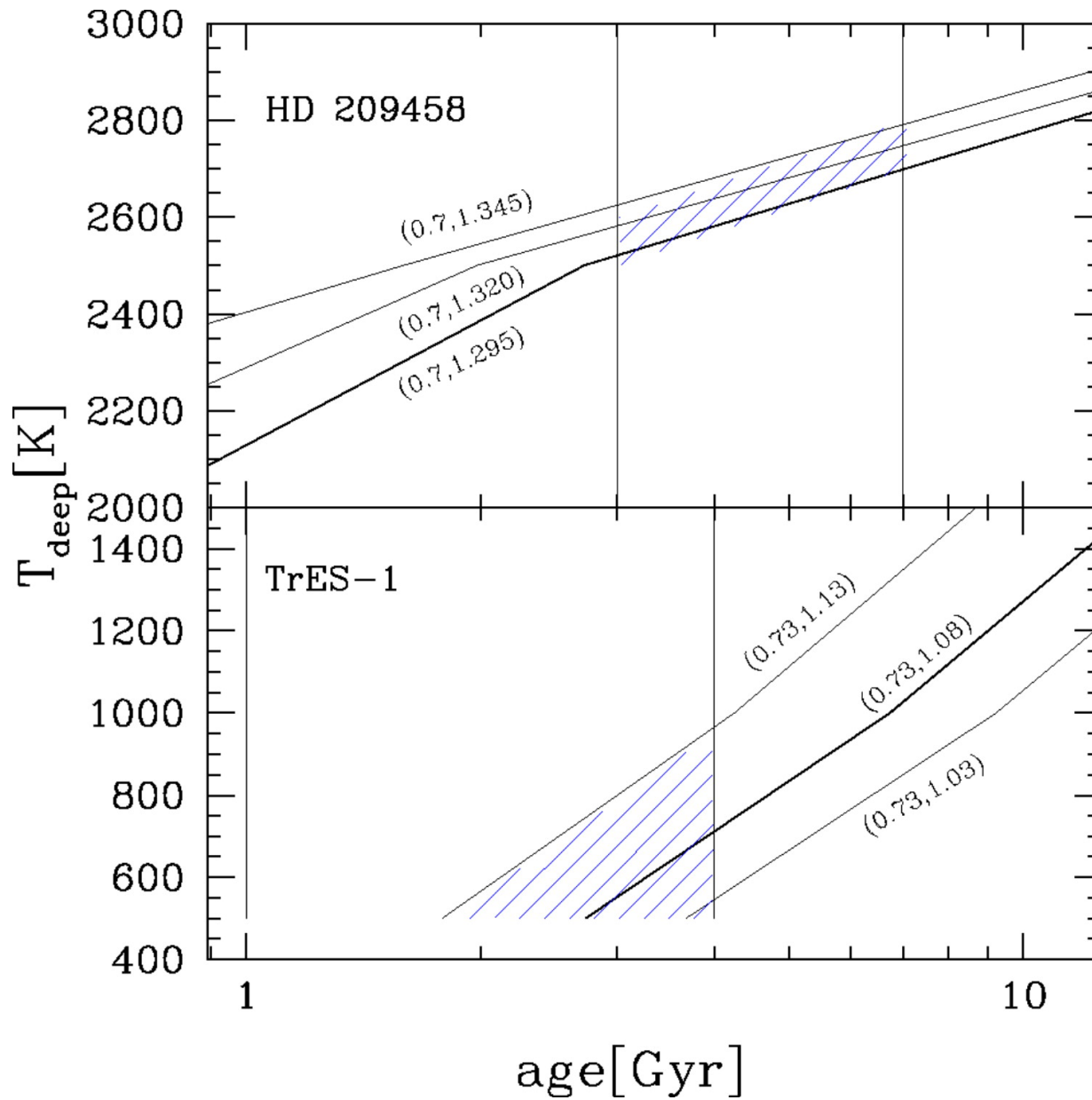
Fig. 17. from Thermal Structure and Radius Evolution of Irradiated Gas Giant Planets Arras & Bildsten 2006 ApJ 650 394 doi:10.1086/506011 https://dx.doi.org/10.1086/506011
