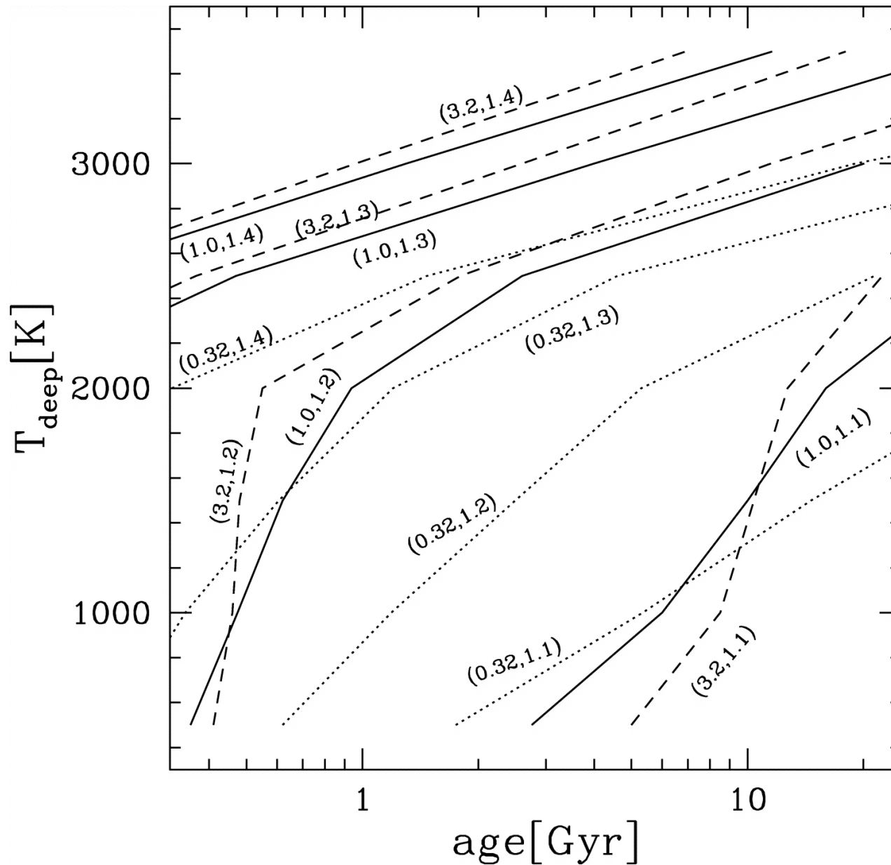
Fig. 15. from Thermal Structure and Radius Evolution of Irradiated Gas Giant Planets Arras & Bildsten 2006 ApJ 650 394 doi:10.1086/506011 https://dx.doi.org/10.1086/506011 © 2006. The American Astronomical Society. All rights reserved. Printed in U.S.A.
