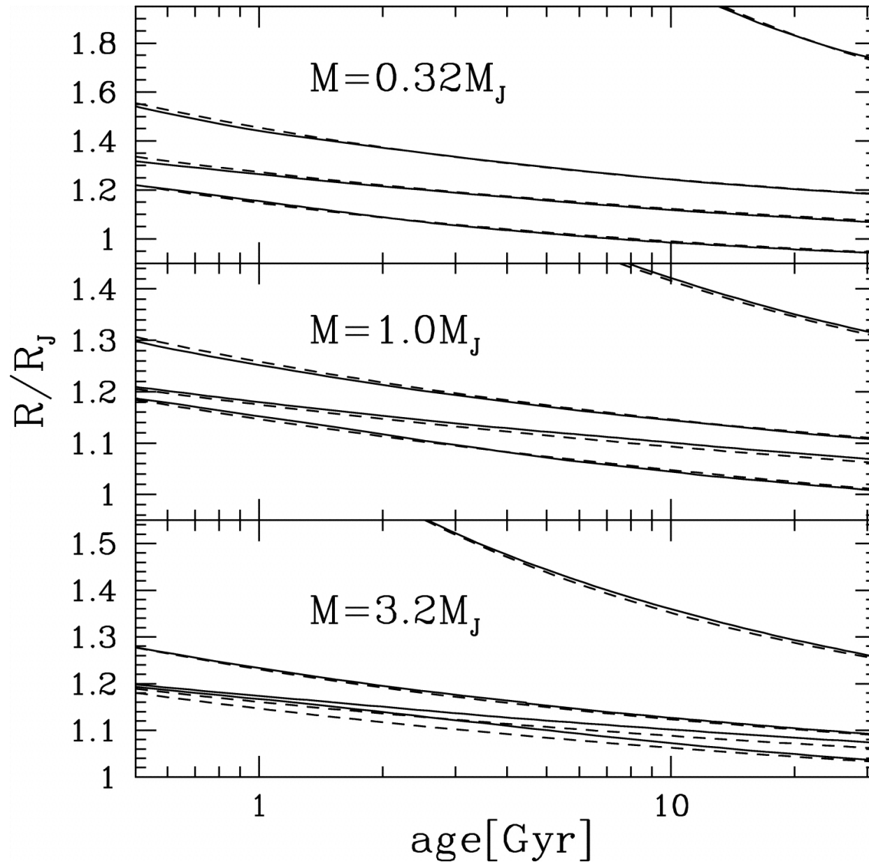
Fig. 14. from Thermal Structure and Radius Evolution of Irradiated Gas Giant Planets Arras & Bildsten 2006 ApJ 650 394 doi:10.1086/506011 https://dx.doi.org/10.1086/506011 © 2006. The American Astronomical Society. All rights reserved. Printed in U.S.A.
