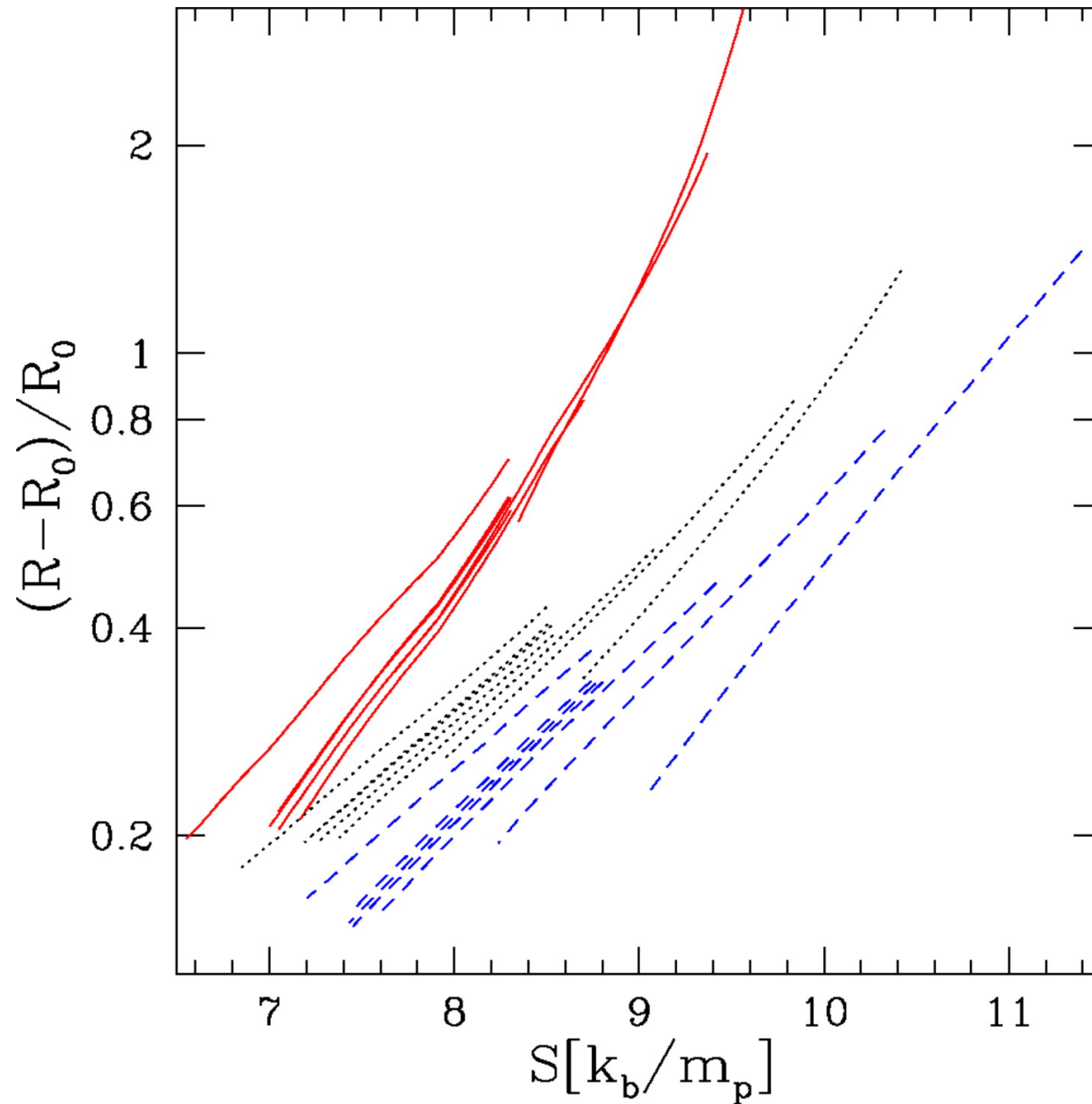
Fig. 13. from Thermal Structure and Radius Evolution of Irradiated Gas Giant Planets Arras & Bildsten 2006 ApJ 650 394 doi:10.1086/506011 https://dx.doi.org/10.1086/506011 © 2006. The American Astronomical Society. All rights reserved. Printed in U.S.A.
