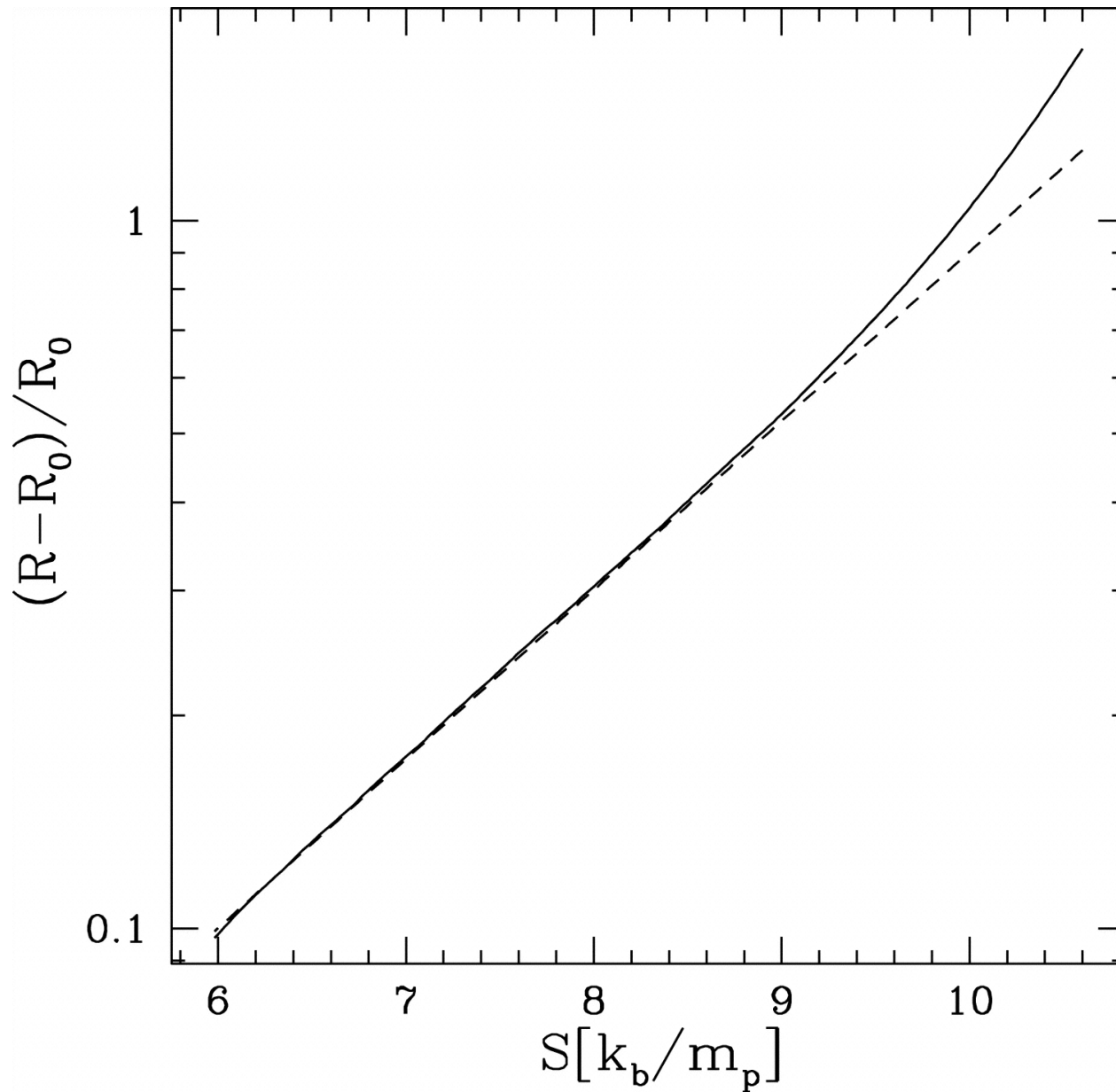
Fig. 12. from Thermal Structure and Radius Evolution of Irradiated Gas Giant Planets Arras & Bildsten 2006 ApJ 650 394 doi:10.1086/506011 https://dx.doi.org/10.1086/506011 © 2006. The American Astronomical Society. All rights reserved. Printed in U.S.A.
