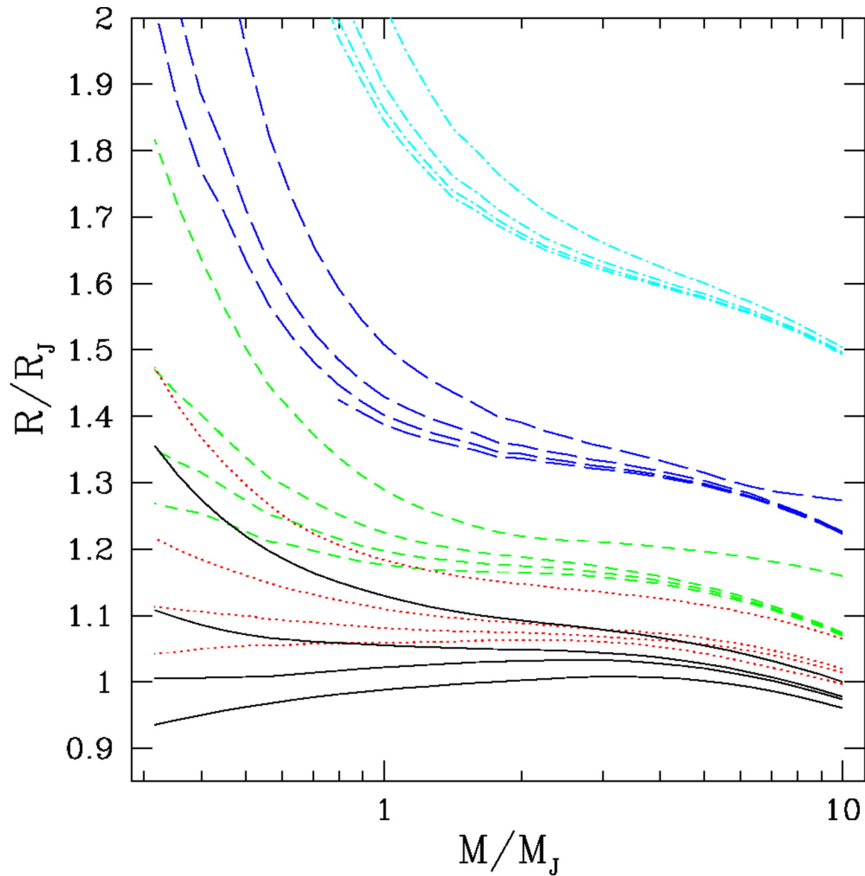
Fig. 10. from Thermal Structure and Radius Evolution of Irradiated Gas Giant Planets Arras & Bildsten 2006 ApJ 650 394 doi:10.1086/506011 https://dx.doi.org/10.1086/506011
