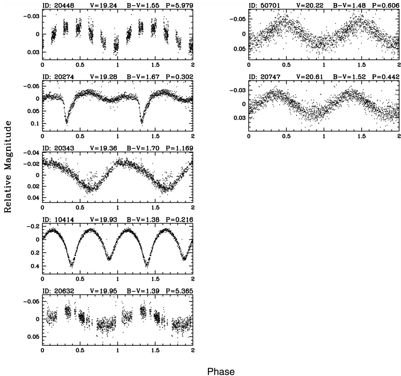
Fig. 5. from Survey for Transiting Extrasolar Planets in Stellar Systems. IV. Variables in the Field of NGC 1245 Pepper & Burke 2006 AJ 132 1177 doi:10.1086/505942 https://dx.doi.org/10.1086/505942
