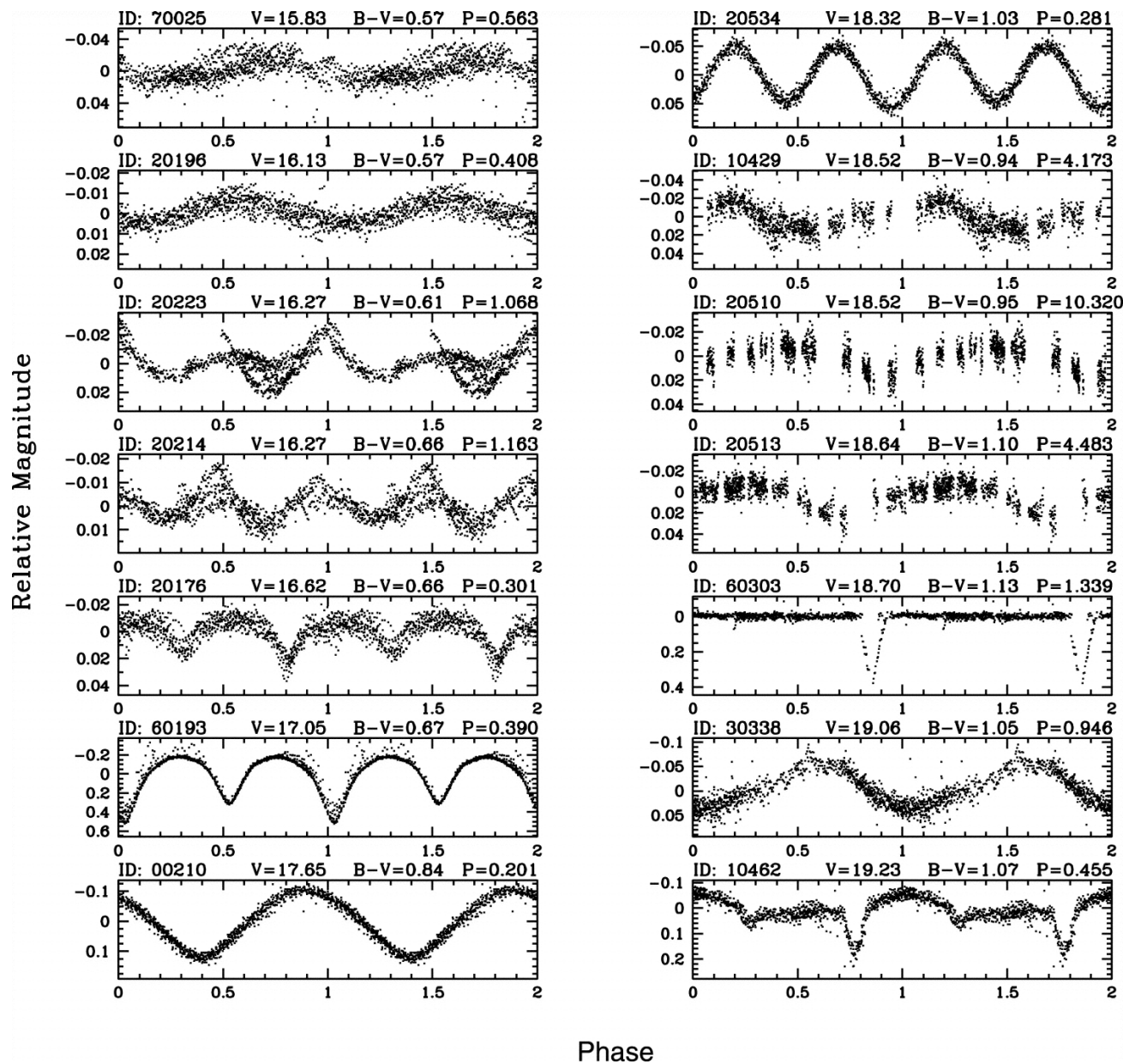
Fig. 2. from Survey for Transiting Extrasolar Planets in Stellar Systems. IV. Variables in the Field of NGC 1245 Pepper & Burke 2006 AJ 132 1177 doi:10.1086/505942 https://dx.doi.org/10.1086/505942
