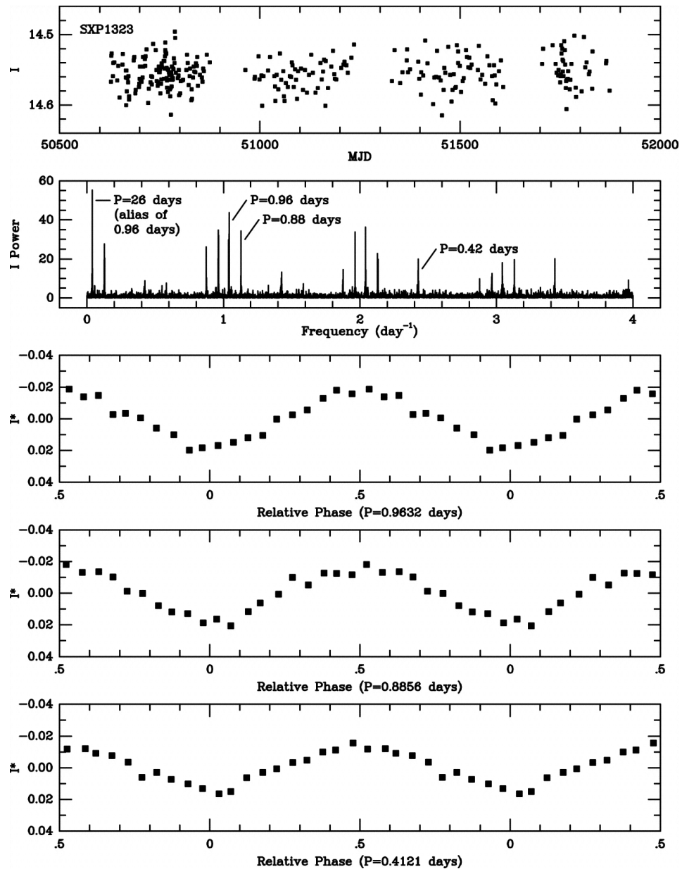
Fig. 6. from Photometric Variability of Be/XRay Pulsar Binaries in the Small Magellanic Cloud Schmidtke & Cowley 2006 AJ 132 919 doi:10.1086/505752 https://dx.doi.org/10.1086/505752
