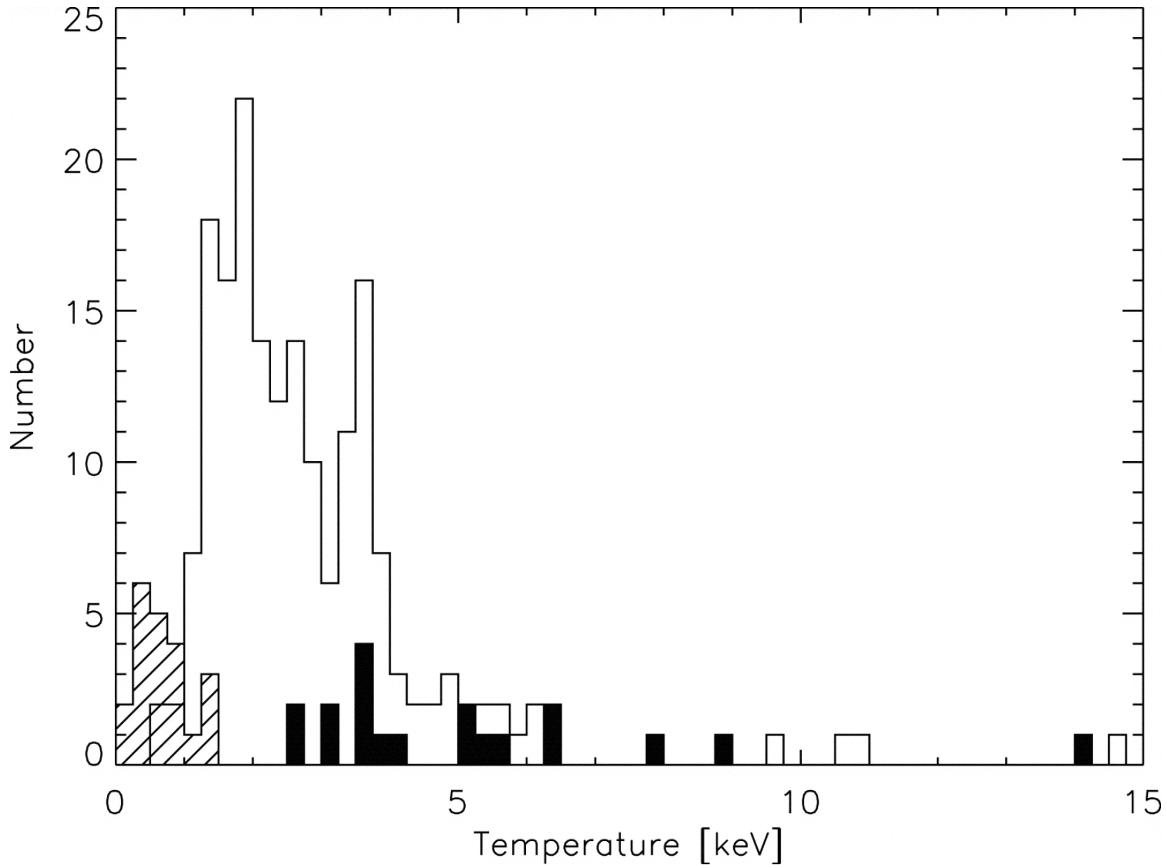
Fig. 9. from XRay and Infrared Point Source Identification and Characteristics in the Embedded, Massive StarForming Region RCW 38 Wolk et al. 2006 AJ 132 1100 doi:10.1086/505704 https://dx.doi.org/10.1086/505704
