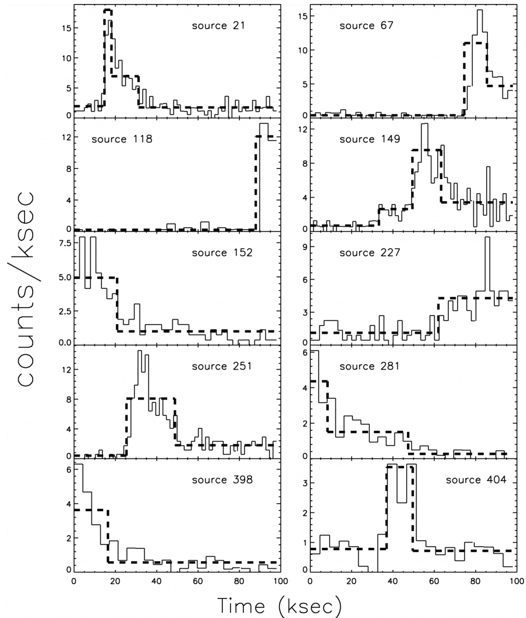
Fig. 6. from XRay and Infrared Point Source Identification and Characteristics in the Embedded, Massive StarForming Region RCW 38 Wolk et al. 2006 AJ 132 1100 doi:10.1086/505704 https://dx.doi.org/10.1086/505704
