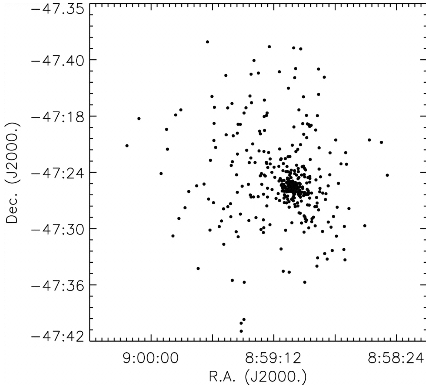
Fig. 4. from XRay and Infrared Point Source Identification and Characteristics in the Embedded, Massive StarForming Region RCW 38 Wolk et al. 2006 AJ 132 1100 doi:10.1086/505704 https://dx.doi.org/10.1086/505704
