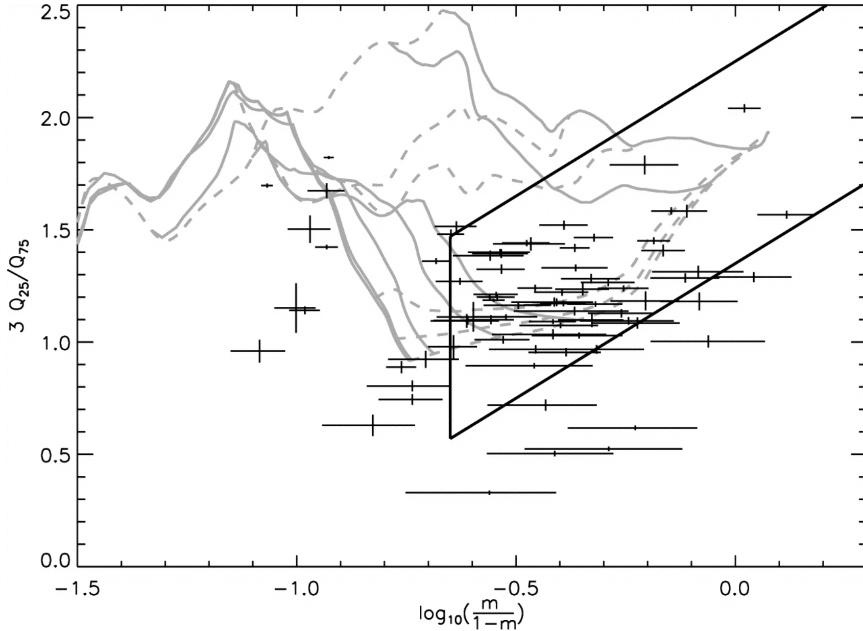
Fig. 3. from XRay and Infrared Point Source Identification and Characteristics in the Embedded, Massive StarForming Region RCW 38 Wolk et al. 2006 AJ 132 1100 doi:10.1086/505704 https://dx.doi.org/10.1086/505704
