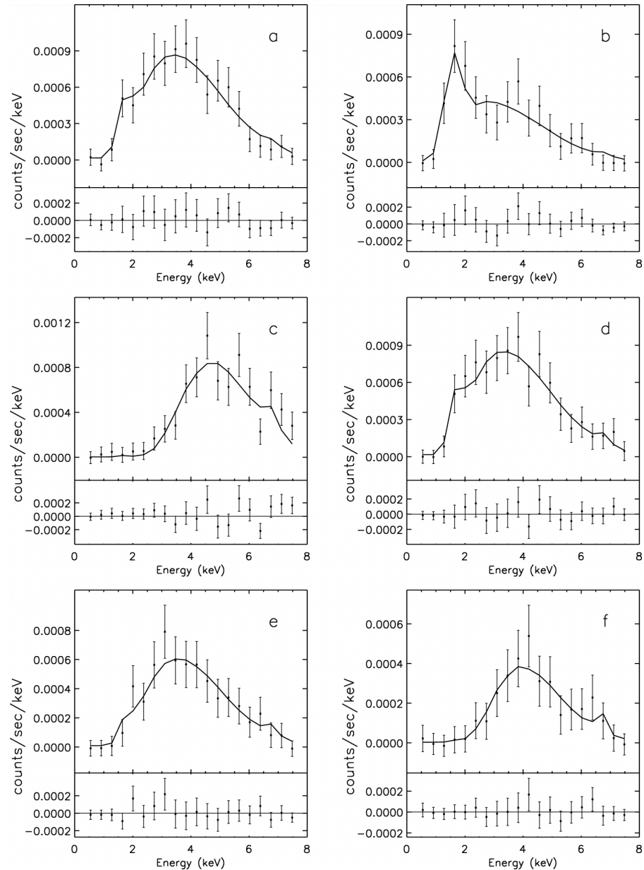
Fig. 20. from XRay and Infrared Point Source Identification and Characteristics in the Embedded, Massive StarForming Region RCW 38 Wolk et al. 2006 AJ 132 1100 doi:10.1086/505704 https://dx.doi.org/10.1086/505704
