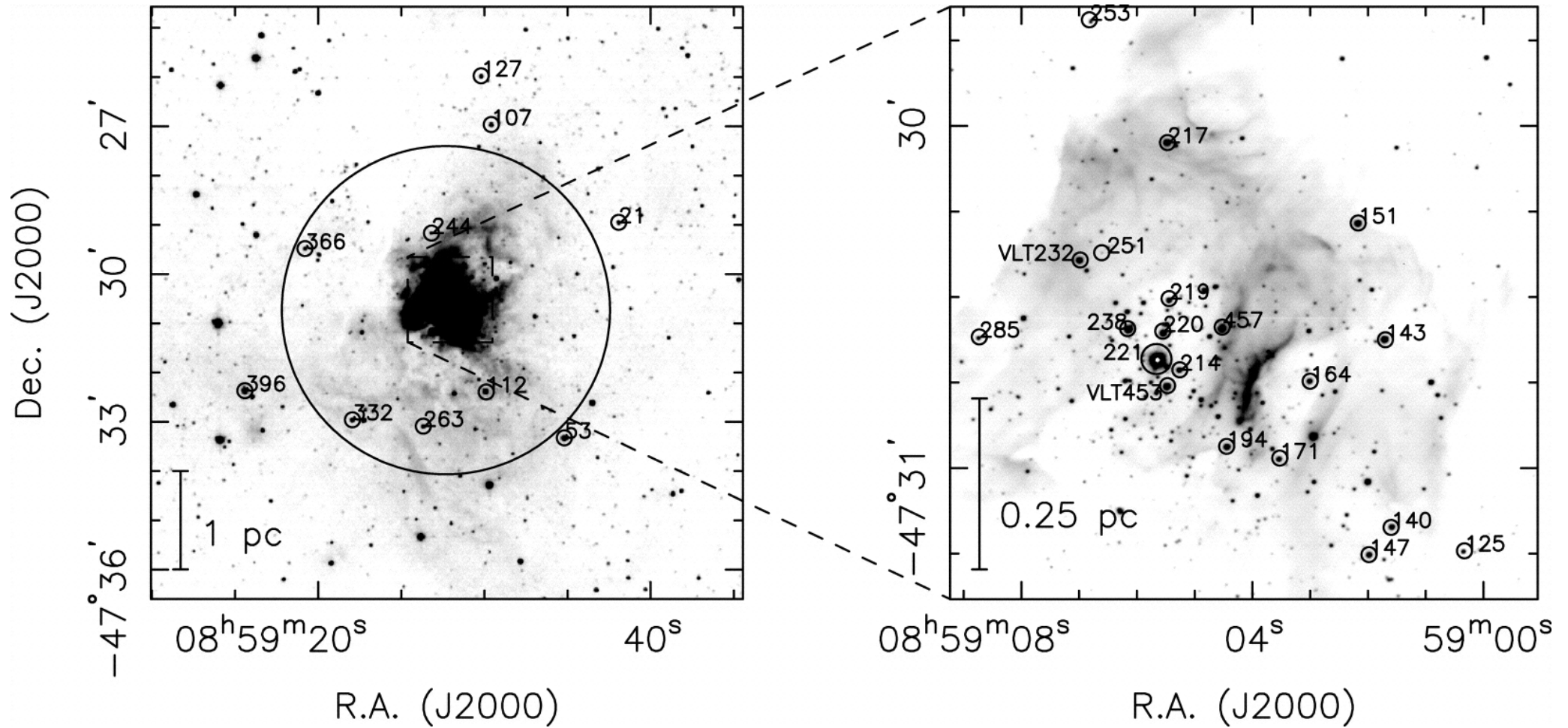
Fig. 18. from XRay and Infrared Point Source Identification and Characteristics in the Embedded, Massive StarForming Region RCW 38 Wolk et al. 2006 AJ 132 1100 doi:10.1086/505704 https://dx.doi.org/10.1086/505704 © 2006. The American Astronomical Society. All rights reserved. Printed in U.S.A.
