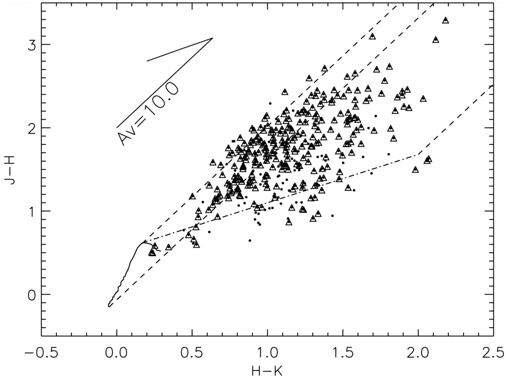
Fig. 17. from XRay and Infrared Point Source Identification and Characteristics in the Embedded, Massive StarForming Region RCW 38 Wolk et al. 2006 AJ 132 1100 doi:10.1086/505704 https://dx.doi.org/10.1086/505704 © 2006. The American Astronomical Society. All rights reserved. Printed in U.S.A.
